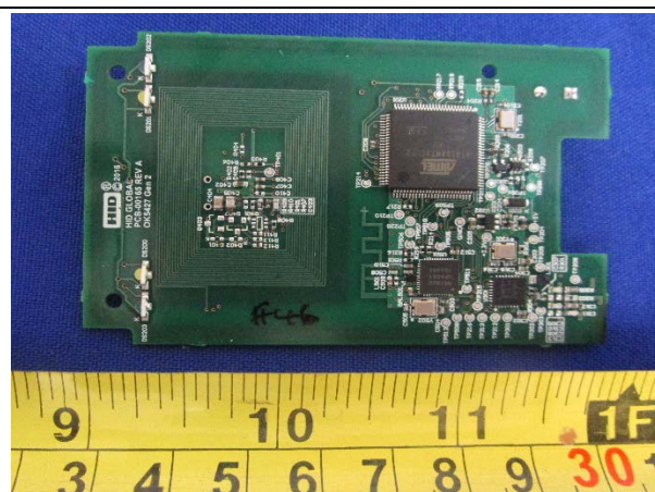
EUT Main PCB – Top View
