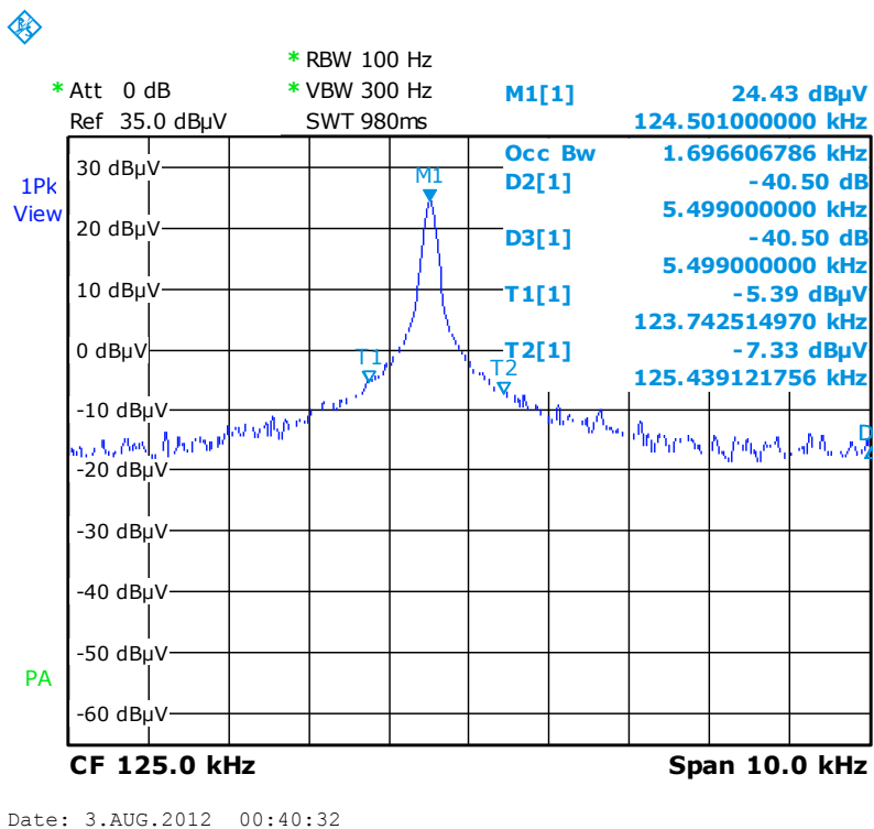
Plots: 125KHz
