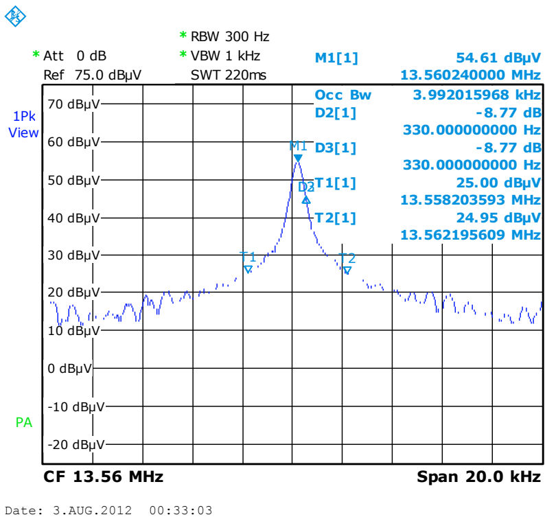
Plots: 13.56 MHz
