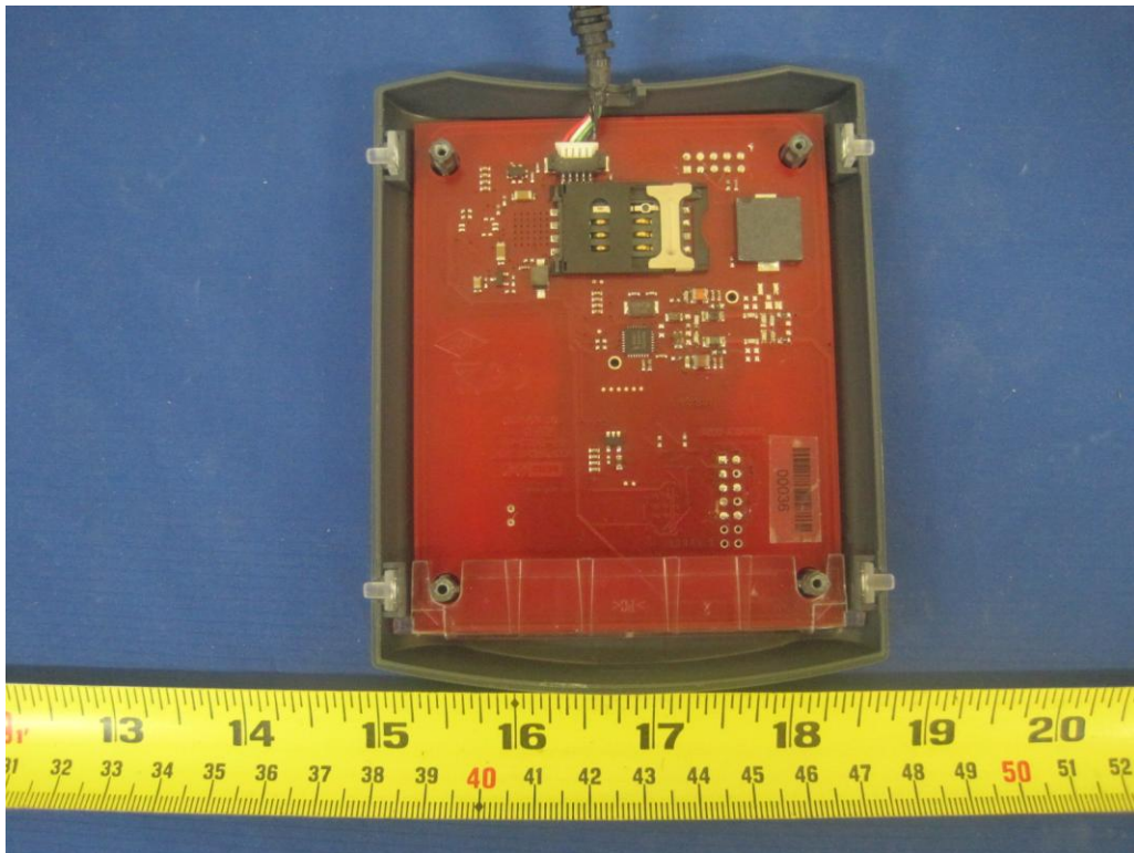
EUT Top View with Chassis off
