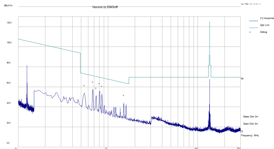
f= 100kHz – 30MHz plot, and loop antenna at 90 degree
