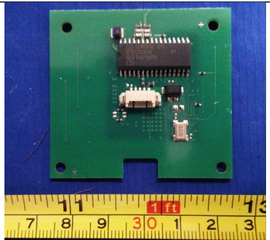
OK5021 PCBA-Bottom View
