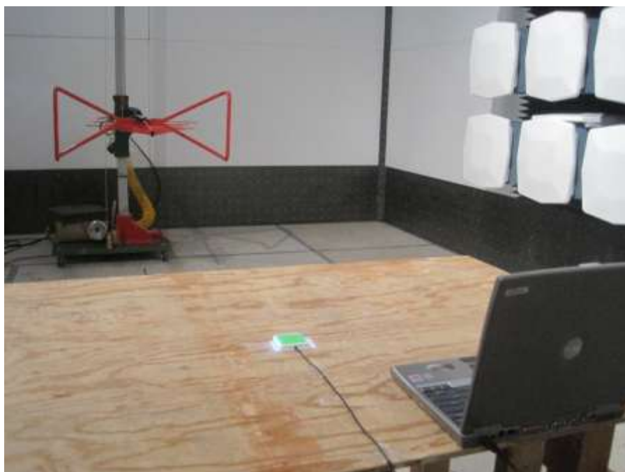
Radiated Emission (>30MHz) – Front View
