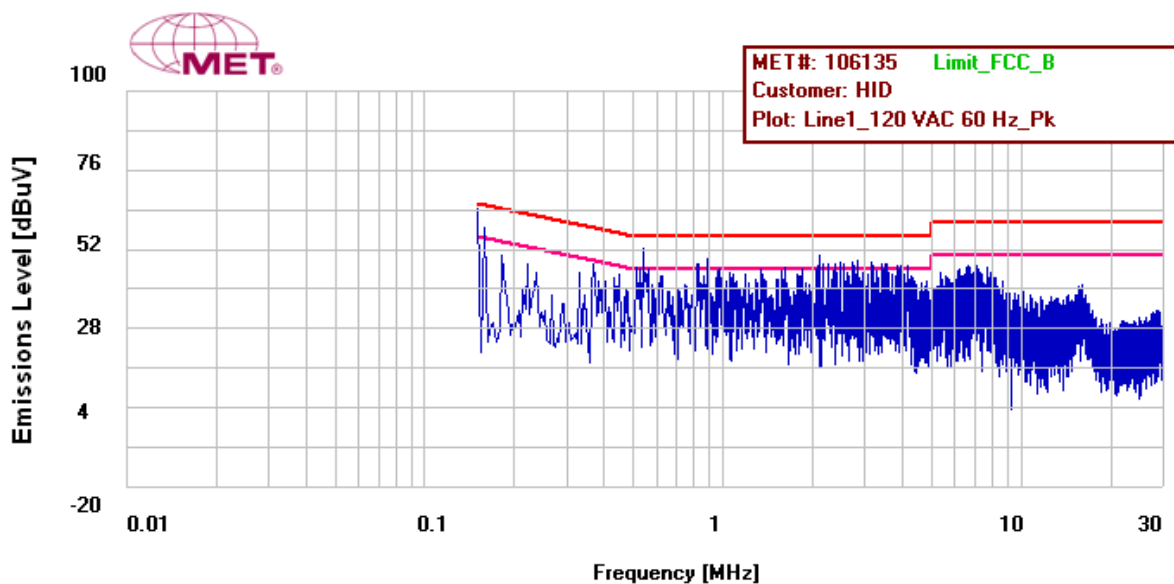
Figure 13. Conducted Emissions, Line Plot
