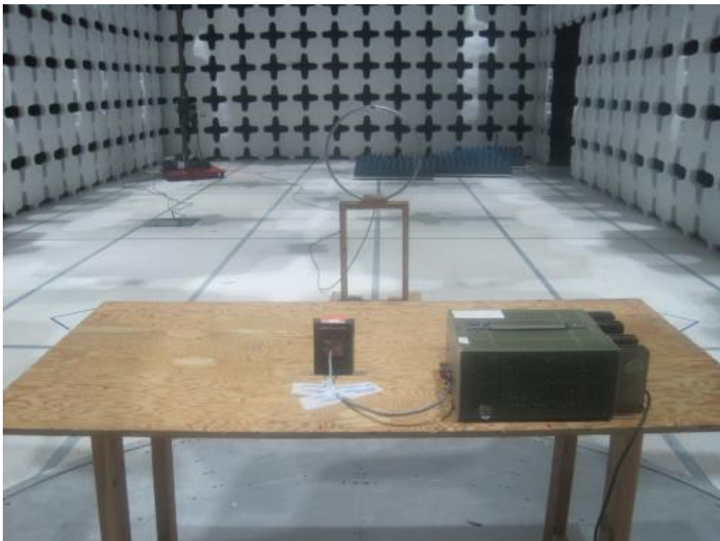
Radiated Emissions (<30MHz) Rear View – Pigtail Connector
