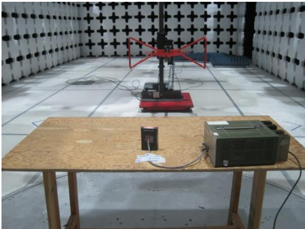
Radiated Emissions (<1GHz) Rear View – Pigtail Connector
