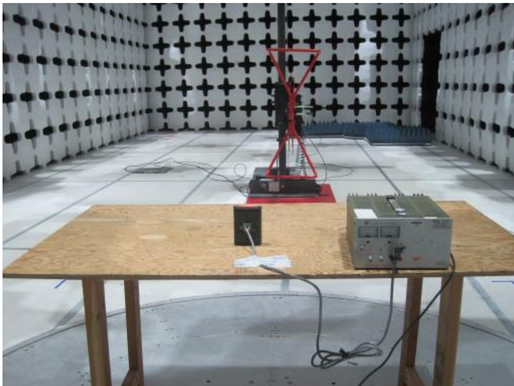
Radiated Emissions (<1GHz) Rear View – Terminal Connector
