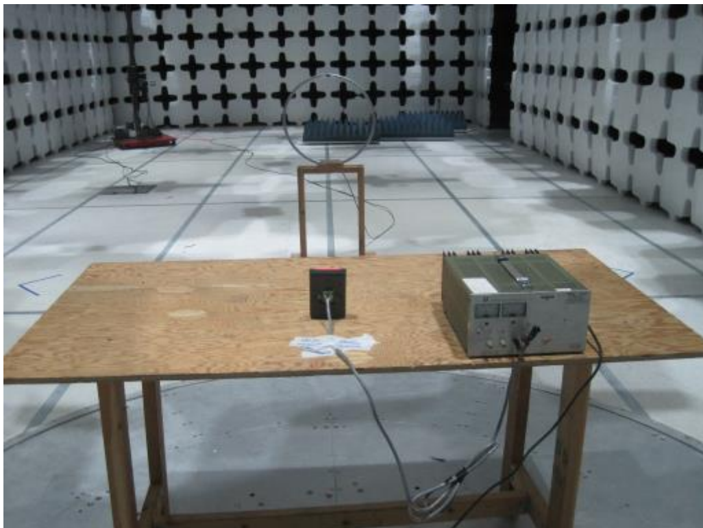
Radiated Emissions (<30MHz) Rear View – Terminal Connector
