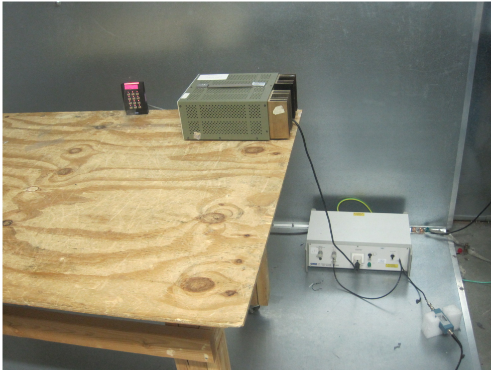
Pigtail cable Conducted Emission Test Setup – Front View
