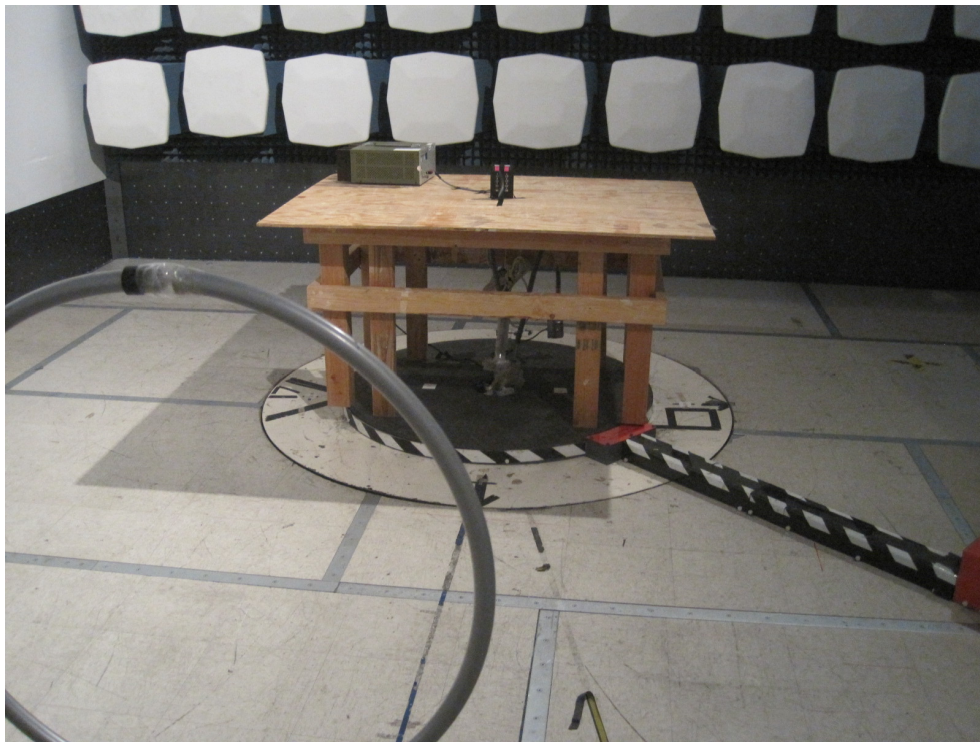
Pigtail cable Radiated Emission<30MHz Test Setup – Front View
