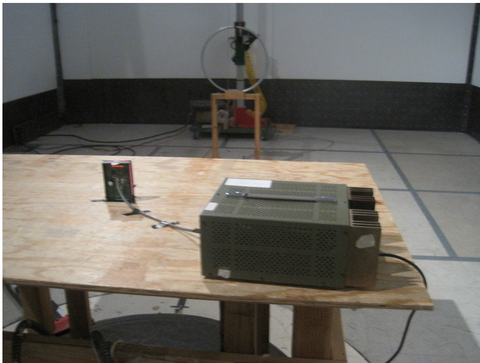
Pigtail cable Radiated Emission<30MHz Test Setup – Rear View
