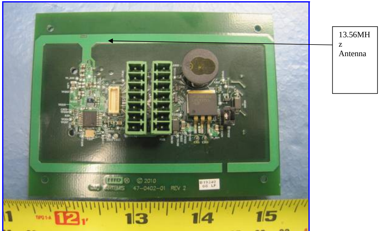
13.56MHz RP Reader Radio Board – Component View
