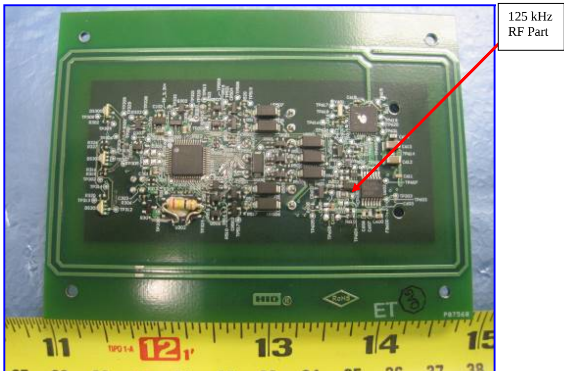
125kHz RP Reader Radio Board View
