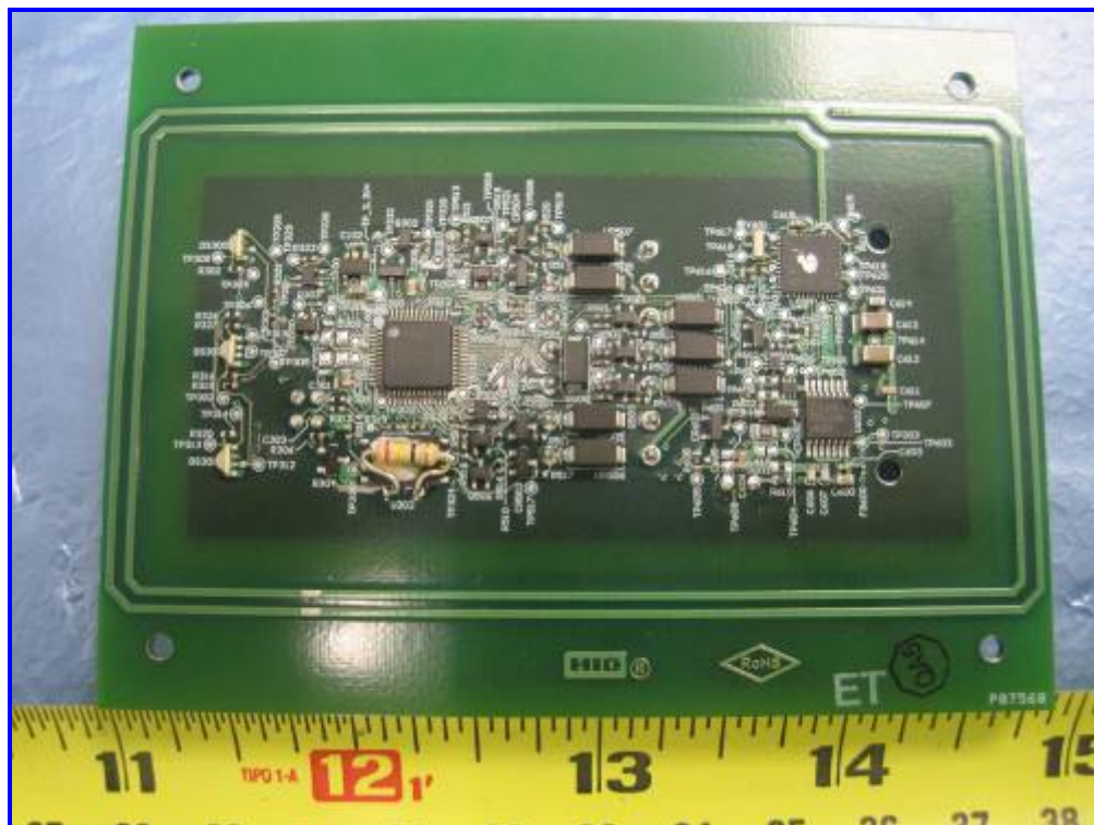
13.56MHz RP Reader Radio Board – Solder View
