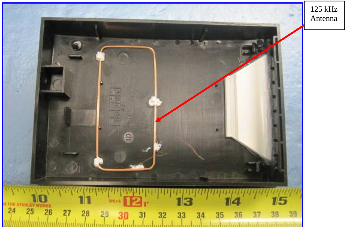
125KHz RP Reader Antenna View
