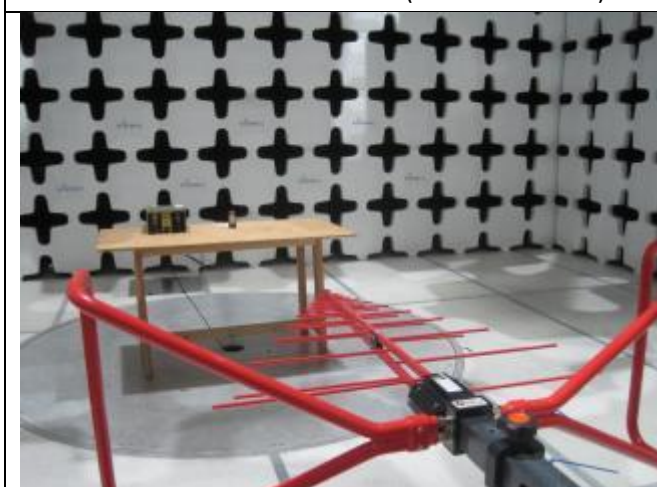
Radiated Emissions (<1GHz) – Front View (Terminal Connector)
