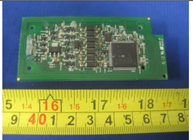
Main PCBA Top View (Terminal Connector)
