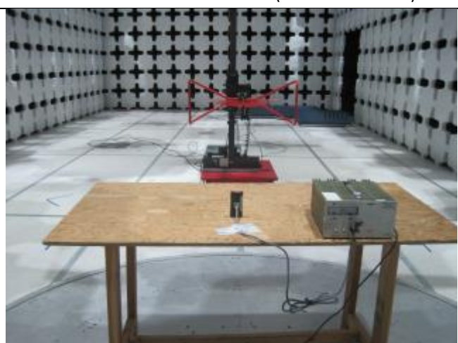
Radiated Emissions (<1GHz) – Rear View (Terminal Connector)
