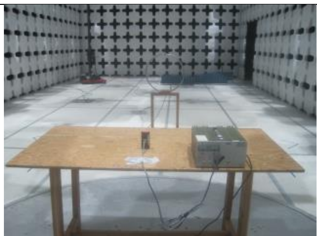
Radiated Emissions (<30MHz) – Rear View (Terminal Connector)
