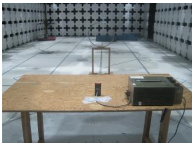
Radiated Emissions (<30MHz) – Rear View (Pigtail Connector)
