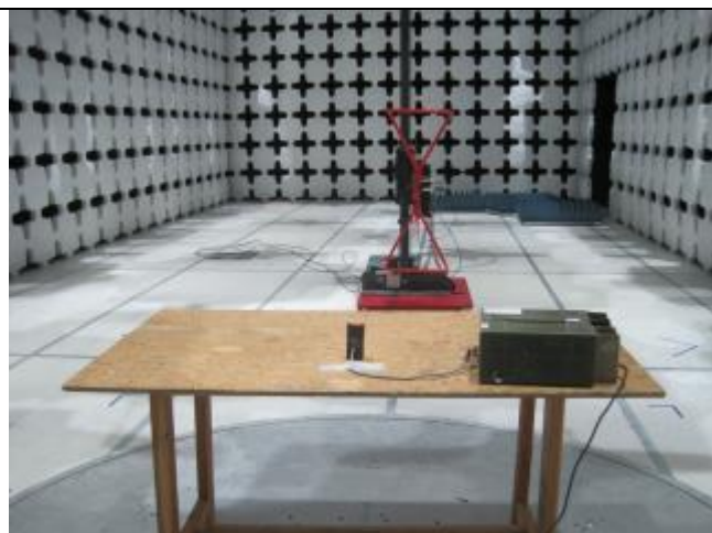
Radiated Emissions (<1GHz) – Rear View (Pigtail Connector)
