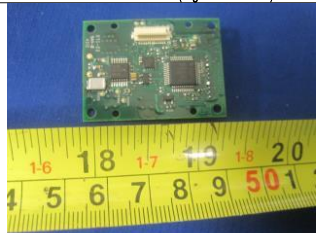
Sub PCBA Bottom View (Pigtail Connector)
