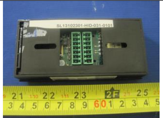
Rear View (Terminal Connector)
