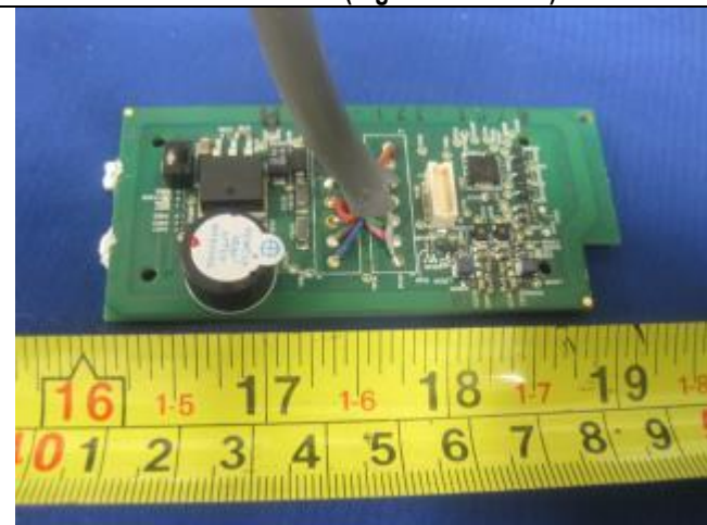
Main PCBA Bottom View (Pigtail Connector)
