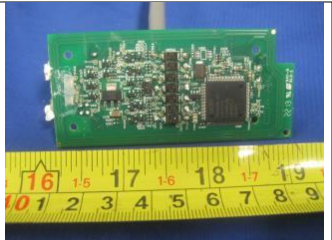
Main PCBA Top View (Pigtail Connector)
