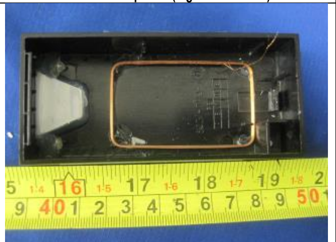
Loop Antenna (Pigtail Connector)
