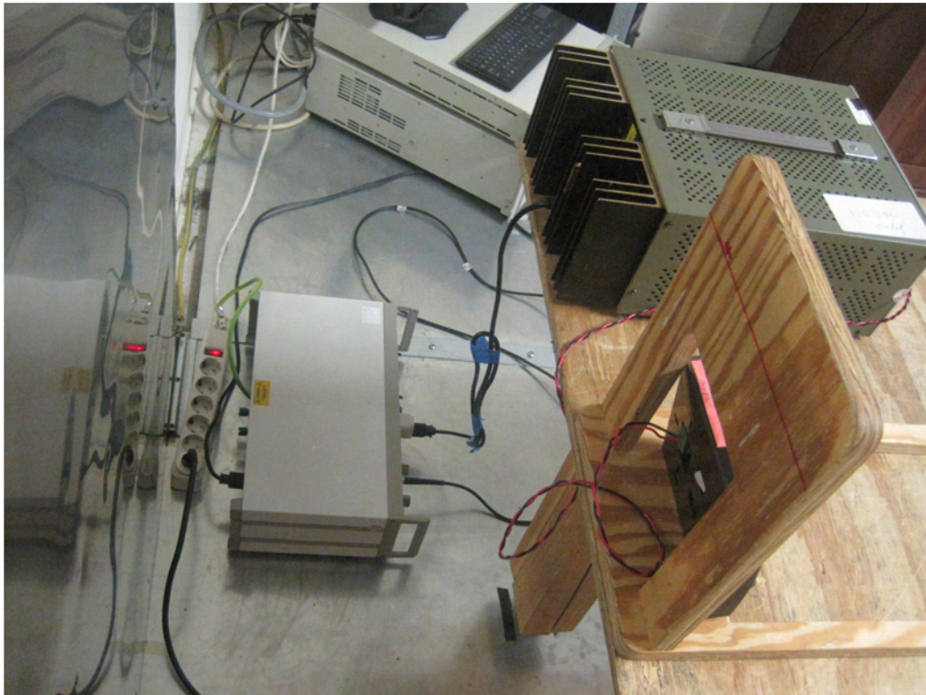
Conducted Emission Test Setup – Rear View
