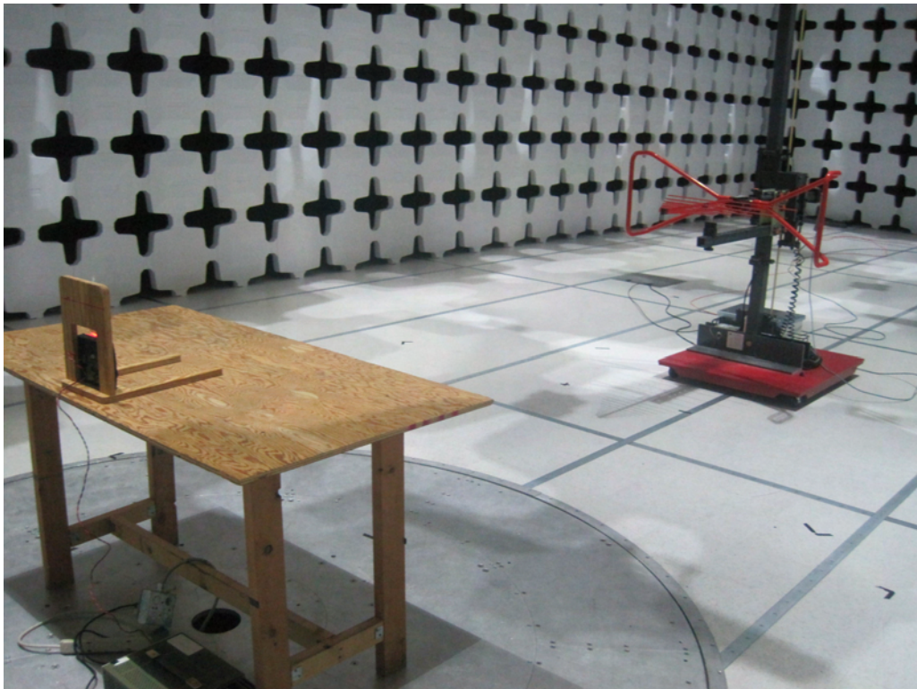
Radiated Emission>30MHz Test Setup – Rear View
