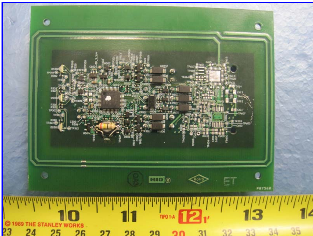
13.56MHz R Reader Radio Board – Solder View
