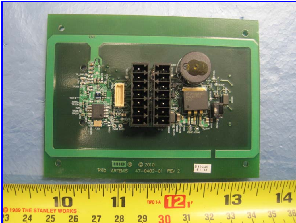
13.56MHz R Reader Radio Board – Component View
