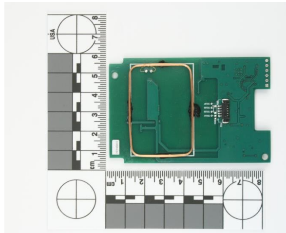
PCBA Bottom View
