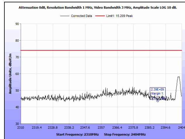
Plot 22. Radiated Restricted Band Edge, 2.402 GHz, Peak – Vertical
