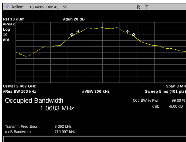
Plot 3. 6 dB Occupied Bandwidth, Low Channel
