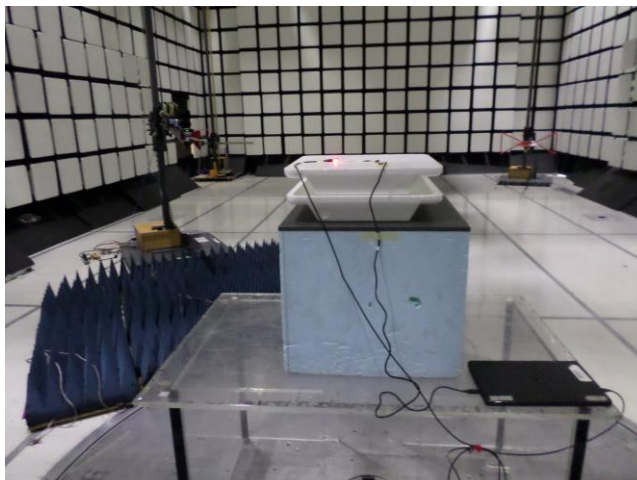
Photograph 9. Radiated Emissions, Above 1 GHz, Rear
