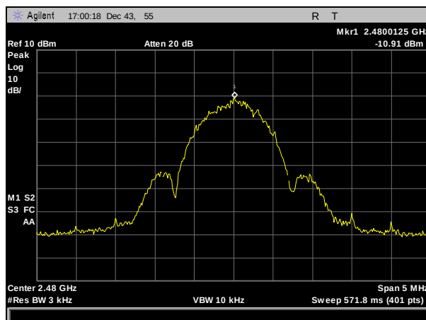
Plot 35. Peak Power Spectral Density, High Channel
