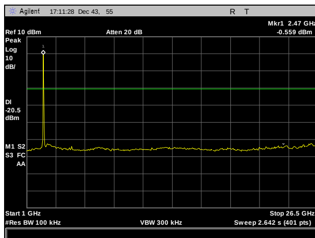
Plot 32. Conducted Spurious Emissions, High Channel, 1 GHz – 26.5 GHz
