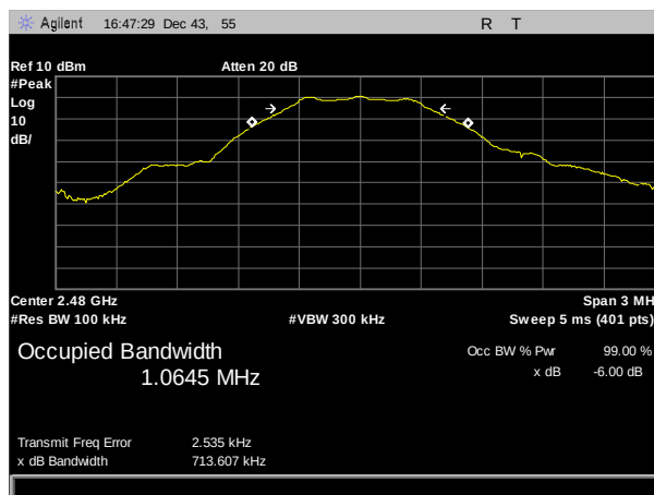
Plot 5. 6 dB Occupied Bandwidth, High Channel
