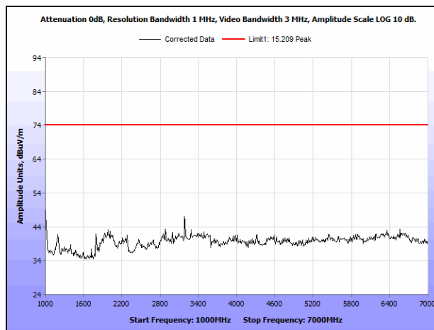
Plot 14. Radiated Spurious Emissions, 1 – 7 GHz, Peak – Vertical
