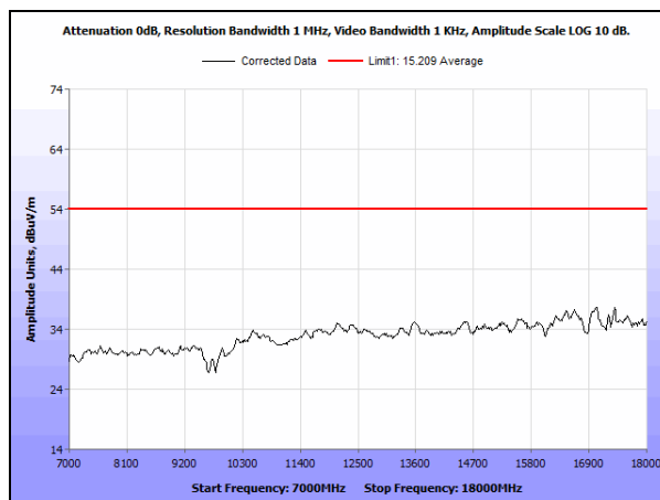
Plot 15. Radiated Spurious Emissions, 7 - 18 GHz, Average – Horizontal
