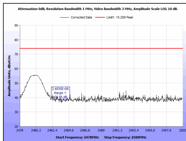
Plot 26. Radiated Restricted Band Edge, 2.480 GHz, Peak - Vertical
