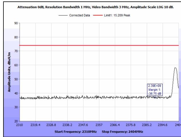
Plot 21. Radiated Restricted Band Edge, 2.402 GHz, Peak - Horizontal
