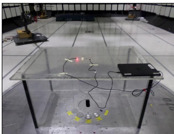
Photograph 6. Radiated Spurious Emissions, Test Setup – Below 1 GHz (Rear)
