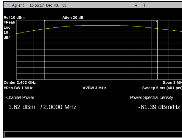
Plot 6. Peak Power Output, Low Channel
