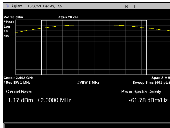
Plot 7. Peak Power Output, Mid Channel
