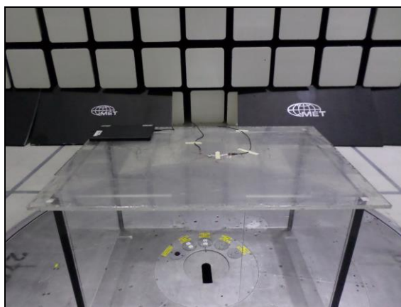
Photograph 5. Radiated Spurious Emissions, Test Setup – Below 1 GHz (Front)
