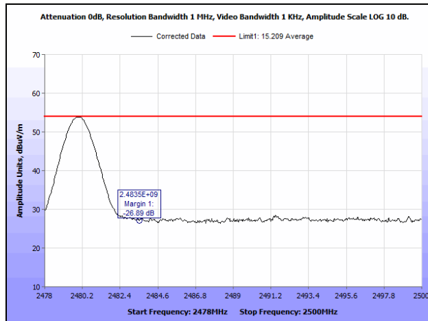
Plot 24. Radiated Restricted Band Edge, 2.480 GHz, Average - Vertical
