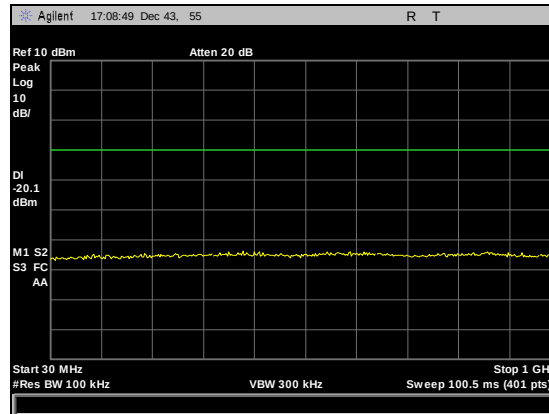
Plot 27. Conducted Spurious Emissions, Low Channel, 30 MHz – 1 GHz
