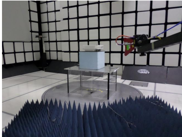
Photograph 7. Radiated Emissions, Above 1 GHz, Antenna
