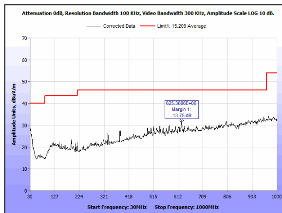
Plot 9. Radiated Spurious Emissions, 30 MHz – 1 GHz - Horizontal
