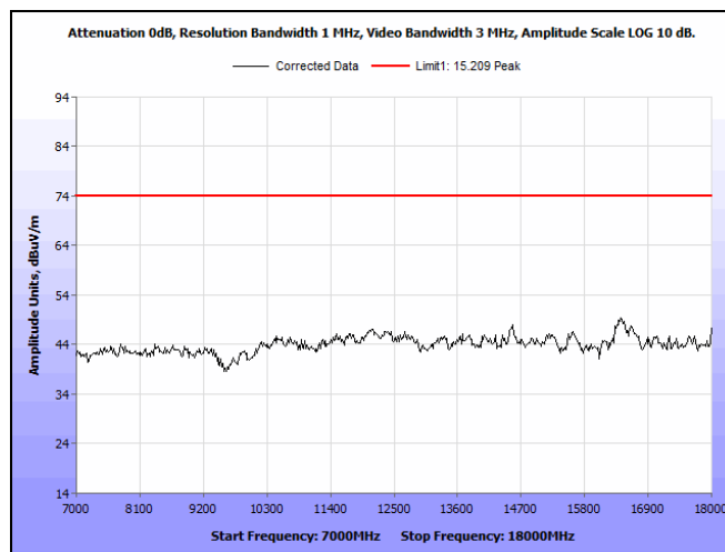
Plot 18. Radiated Spurious Emissions, 7 - 18 GHz, Peak – Vertical
