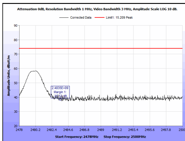
Plot 25. Radiated Restricted Band Edge, 2.480 GHz, Peak - Horizontal
