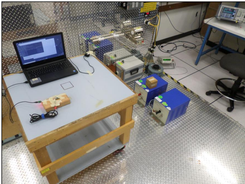
Photograph 1. Conducted Emissions, 15.207(a), Test Setup
