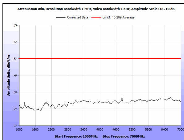
Plot 11. Radiated Spurious Emissions, 1 – 7 GHz, Average – Horizontal
