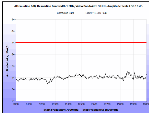
Plot 17. Radiated Spurious Emissions, 7 - 18 GHz, Peak – Horizontal
