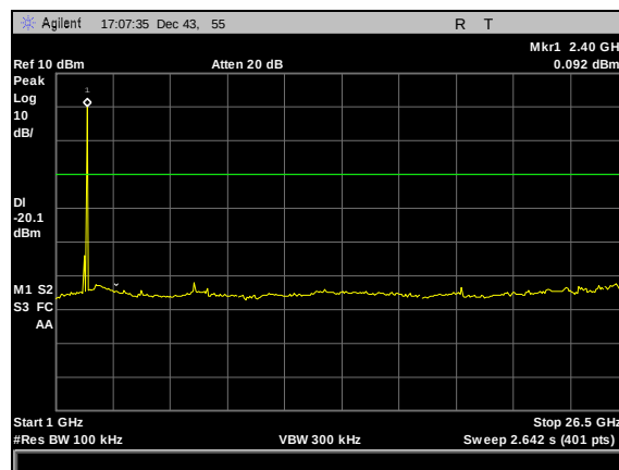
Plot 28. Conducted Spurious Emissions, Low Channel, 1 GHz – 26.5 GHz
