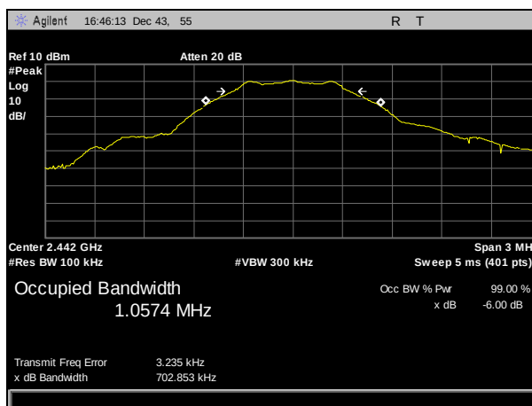
Plot 4. 6 dB Occupied Bandwidth, Mid Channel
