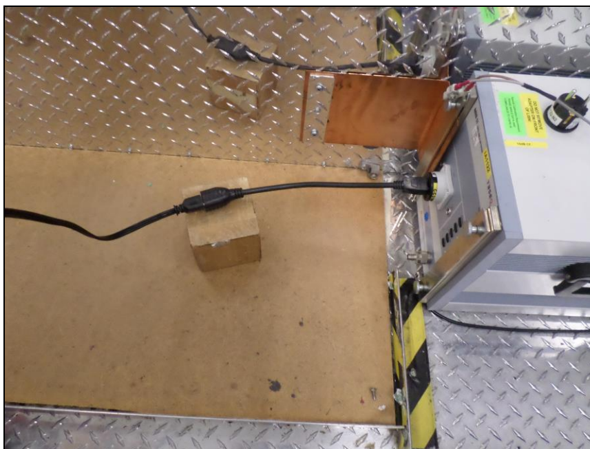
Photograph 2. Conducted Emissions, 15.207(a), LISN Connection
