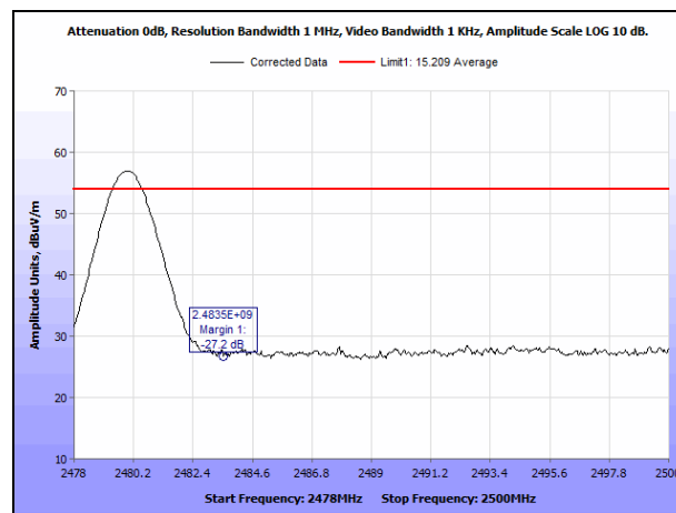
Plot 23. Radiated Restricted Band Edge, 2.480 GHz, Average - Horizontal
