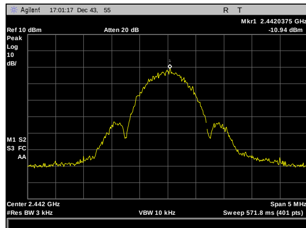
Plot 34. Peak Power Spectral Density, Mid Channel
