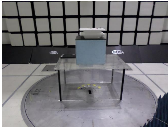
Photograph 8. Radiated Emissions, Above 1 GHz, Front
