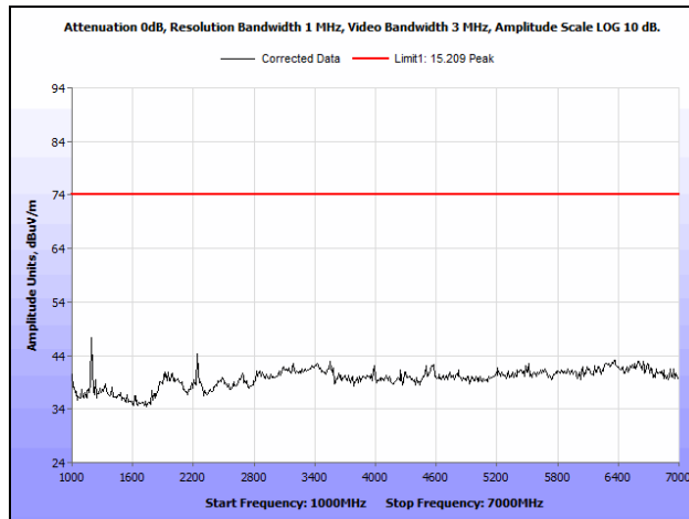
Plot 13. Radiated Spurious Emissions, 1 – 7 GHz, Peak – Horizontal
