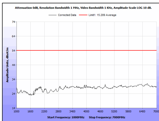
Plot 12. Radiated Spurious Emissions, 1 – 7 GHz, Average – Vertical
