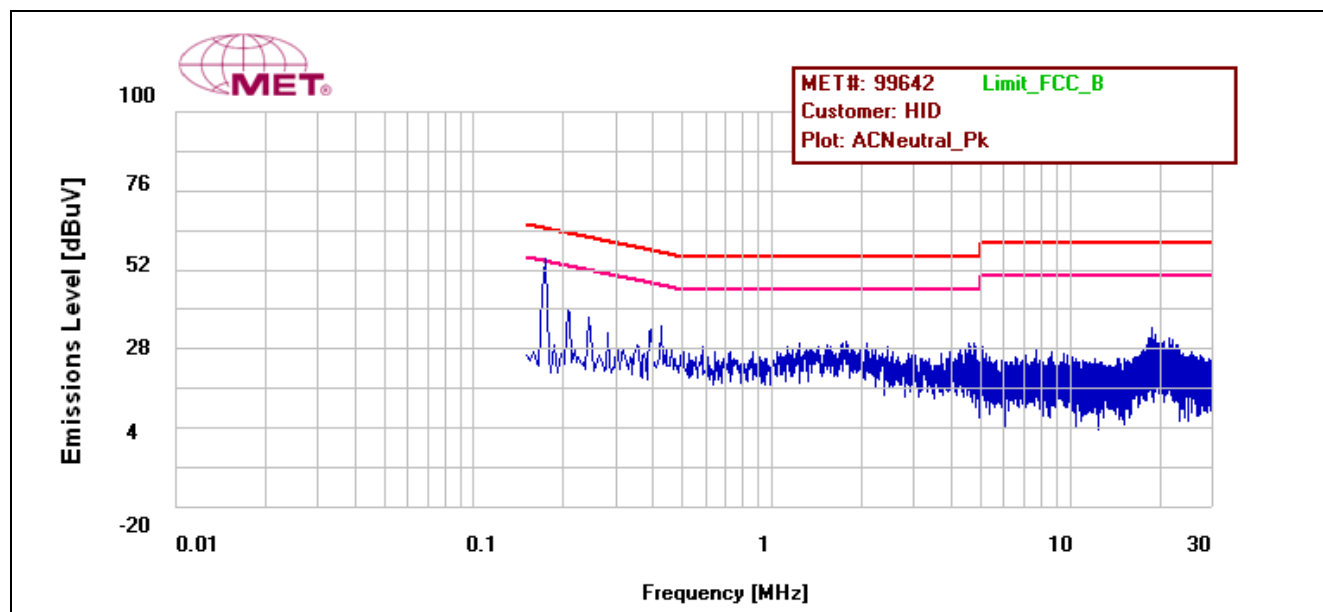
Plot 2. Conducted Emissions, 15.207(a), Neutral Line
