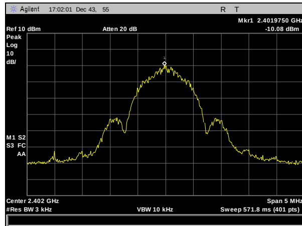
Plot 33. Peak Power Spectral Density, Low Channel
