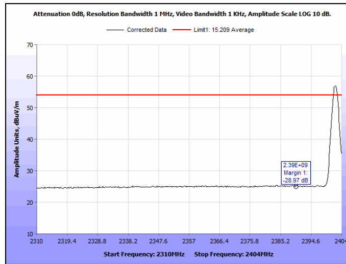
Plot 19. Radiated Restricted Band Edge, 2.402 GHz, Average - Horizontal
