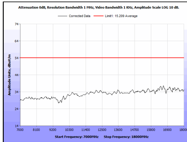
Plot 16. Radiated Spurious Emissions, 7 - 18 GHz, Average – Vertical
