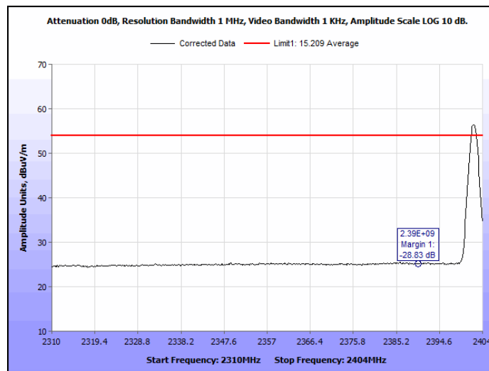
Plot 20. Radiated Restricted Band Edge, 2.402 GHz, Average - Vertical
