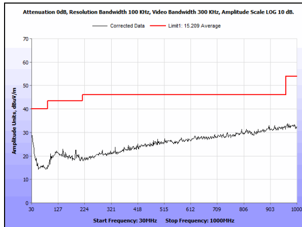
Plot 10. Radiated Spurious Emissions, 30 MHz – 1 GHz - Vertical
