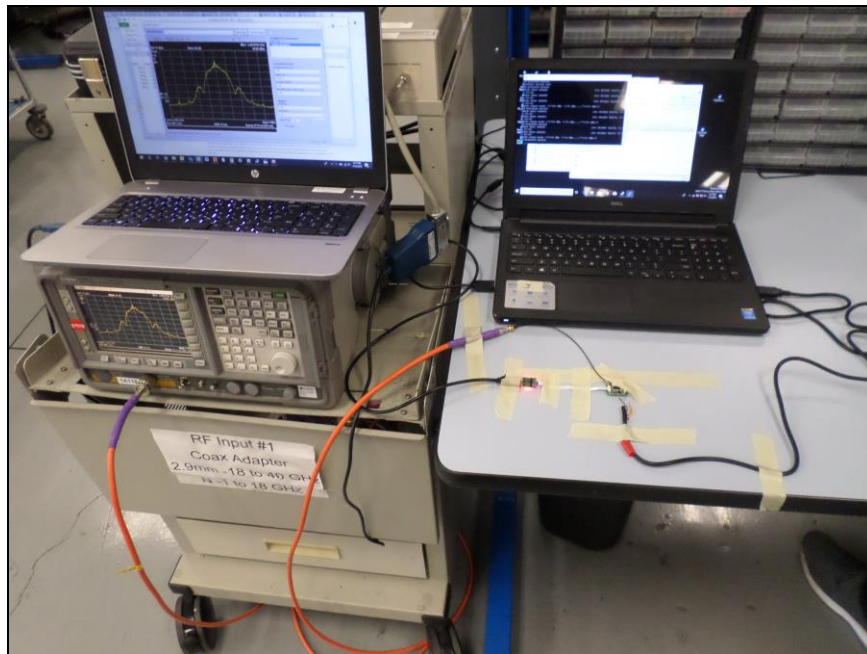
Photograph 3. Conducted Measurement Testing Setup
