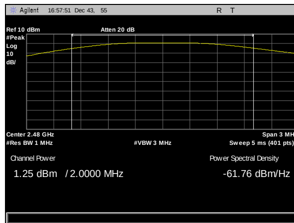
Plot 8. Peak Power Output, High Channel
