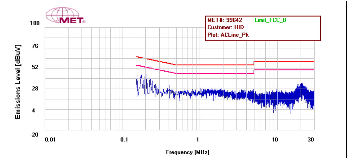
Plot 1. Conducted Emissions, Line
