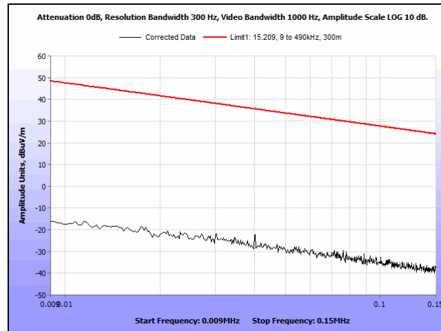
Plot 7. Spurious Emissions, Outside the Bands 13.110 - 14.010 MHz, 0.009 – 0.150 MHz, 90 degrees
