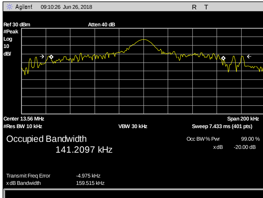
Plot 3. 20 dB Occupied Bandwidth
