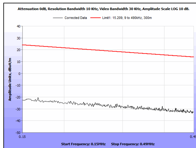
Plot 8. Spurious Emissions, Outside the Bands 13.110 - 14.010 MHz, 0.150 MHz – 0.490 MHz, 0 degrees
