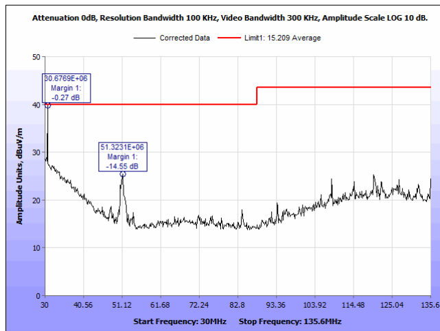
Plot 17. Spurious Emissions, Outside the Bands, 13.110 - 14.010 MHz, 30 MHz – 135.6 MHz, Vertical
