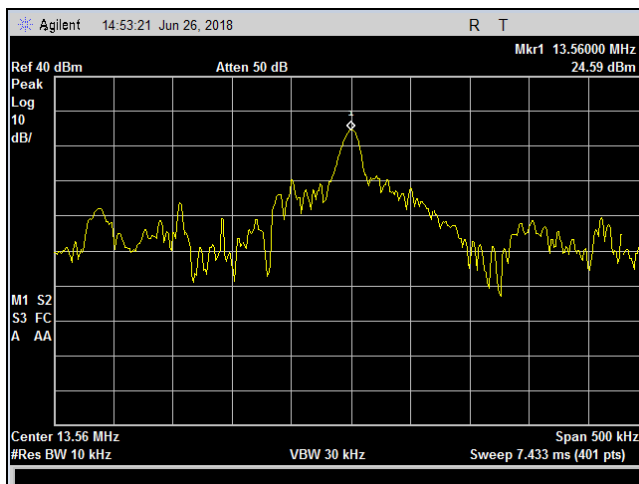
Plot 20. Frequency Stability, Vnom, 50 deg
