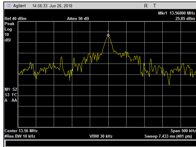
Plot 21. Frequency Stability, +15 pct, 20 deg
