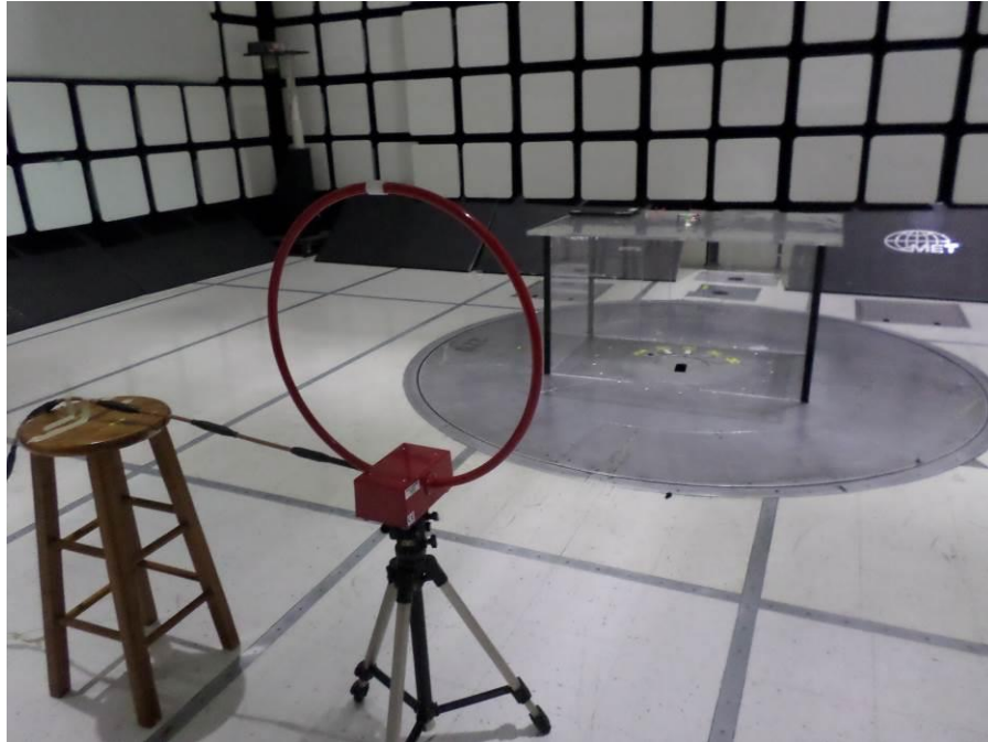
Photograph 4. Field Strength Within the Band 13.553 MHz – 13.567 MHz, 9 kHz – 30 MHz, Antenna
