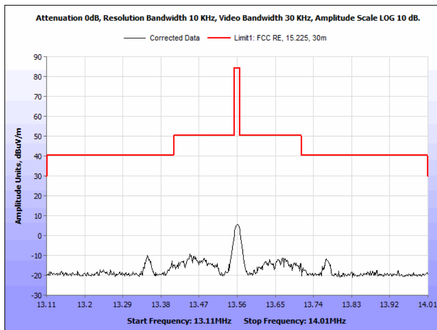
Plot 5. Field Strength Within the Band 13.553 – 13.567 MHz, 90 degrees
