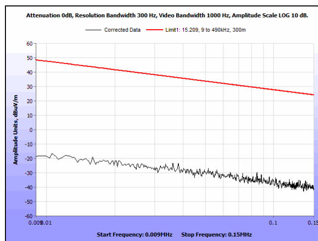
Plot 6. Spurious Emissions, Outside the Bands 13.110 - 14.010 MHz, 0.009 – 0.150 MHz, 0 degrees
