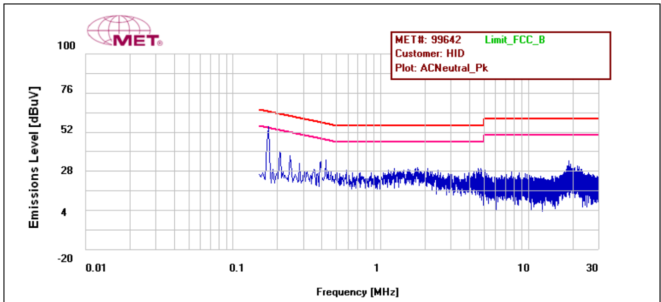
Plot 2. Conducted Emissions, Neutral
