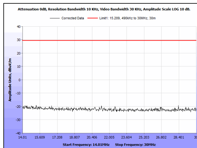
Plot 15. Spurious Emissions, Outside the Bands, 14.010 MHz – 30 MHz, 90 degrees
