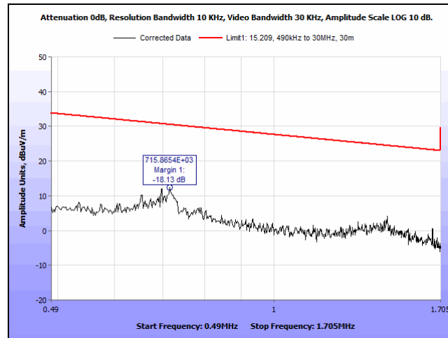
Plot 10. Spurious Emissions, Outside the Bands, 13.110 - 14.010 MHz, 0.490 MHz – 1.705 MHz, 0 degrees
