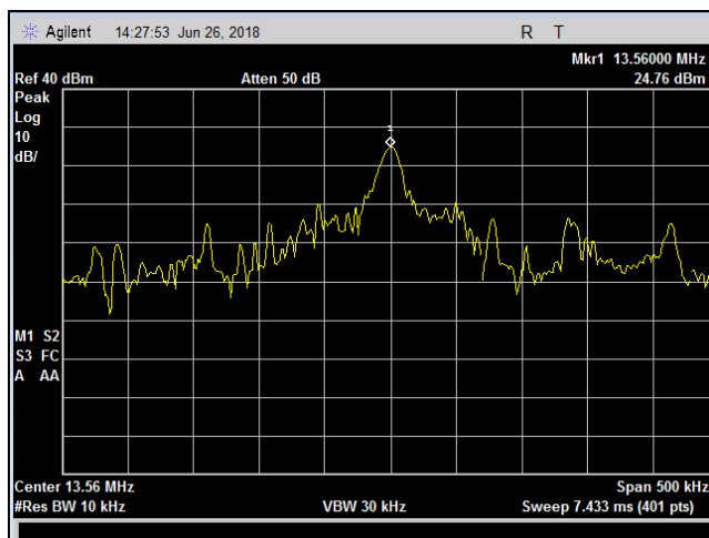
Plot 19. Frequency Stability, Vnom, -20 deg
