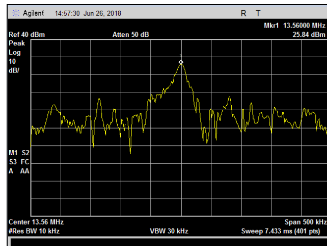
Plot 23. Frequency Stability, +15 pct, 50 deg
