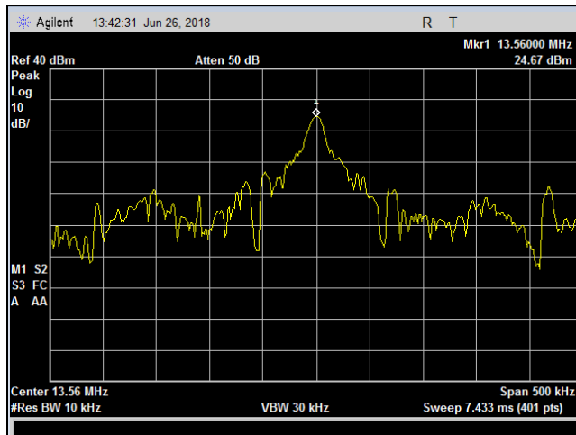
Plot 18. Frequency Stability, Vnom, 20 deg
