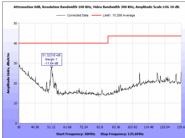
Plot 16. Spurious Emissions, Outside the Bands, 13.110 - 14.010 MHz, 30 MHz – 135.6 MHz, Horizontal
