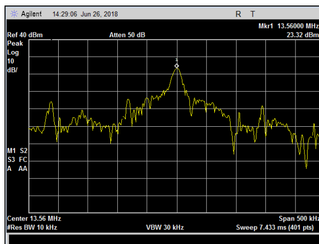
Plot 25. Frequency Stability, -15 pct, -20 deg
