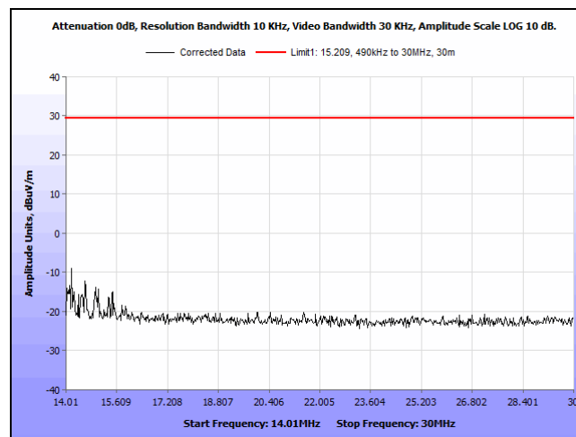
Plot 14. Spurious Emissions, Outside the Bands, 14.010 MHz – 30 MHz, 0 degrees
