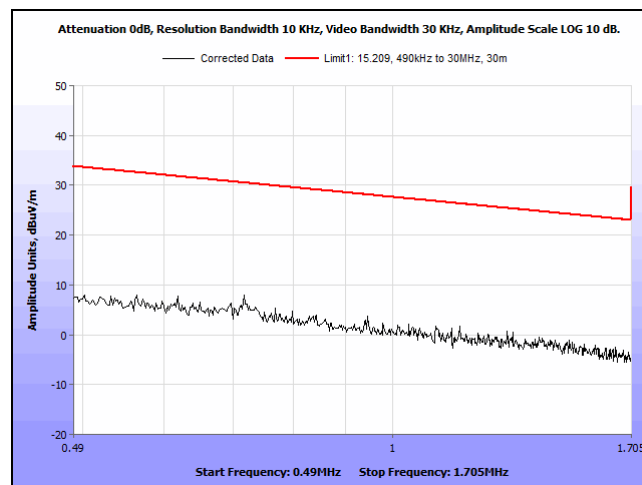
Plot 11. Spurious Emissions, Outside the Bands, 13.110 - 14.010 MHz, 0.490 MHz – 1.705 MHz, 90 degrees
