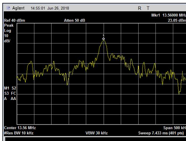
Plot 26. Frequency Stability, -15 pct, 50 deg
