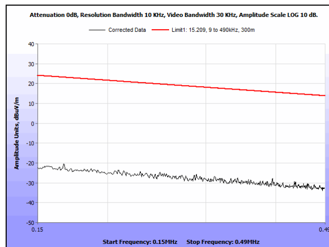
Plot 9. Spurious Emissions, Outside the Bands 13.110 - 14.010 MHz, 0.150 MHz – 0.490 MHz, 90 degrees
