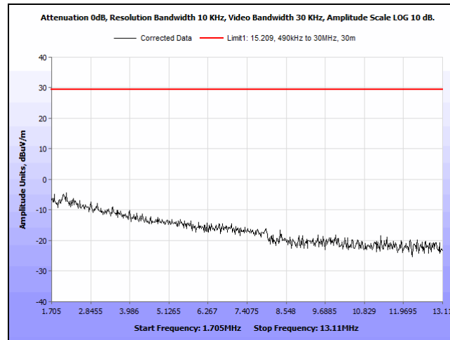
Plot 13. Spurious Emissions, Outside the Bands, 1.705 MHz – 13.11 MHz, 90 degrees
