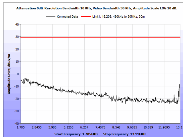
Plot 12. Spurious Emissions, Outside the Bands, 13.110 - 14.010 MHz, 1.705 MHz – 13.11 MHz, 0 degrees
