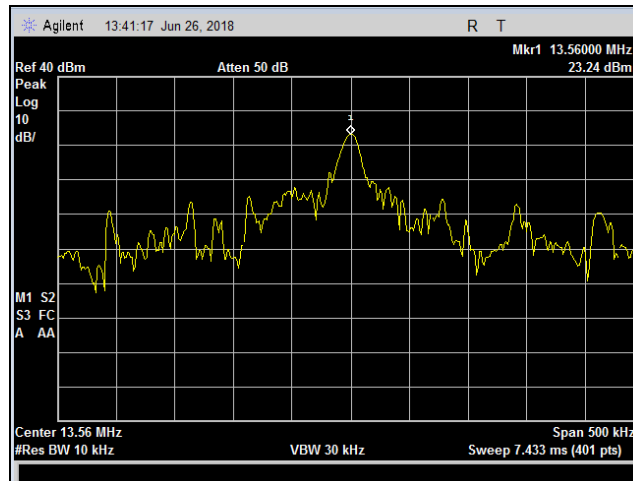
Plot 24. Frequency Stability, -15 pct, 20 deg
