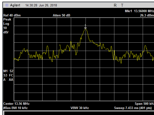
Plot 22. Frequency Stability, +15 pct, -20 deg
