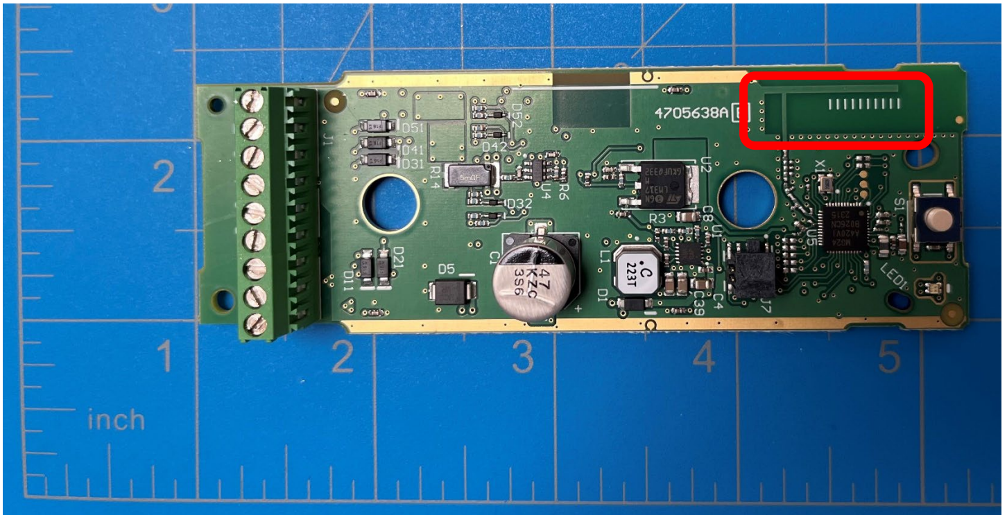
PFIA Antenna Circled in Red
