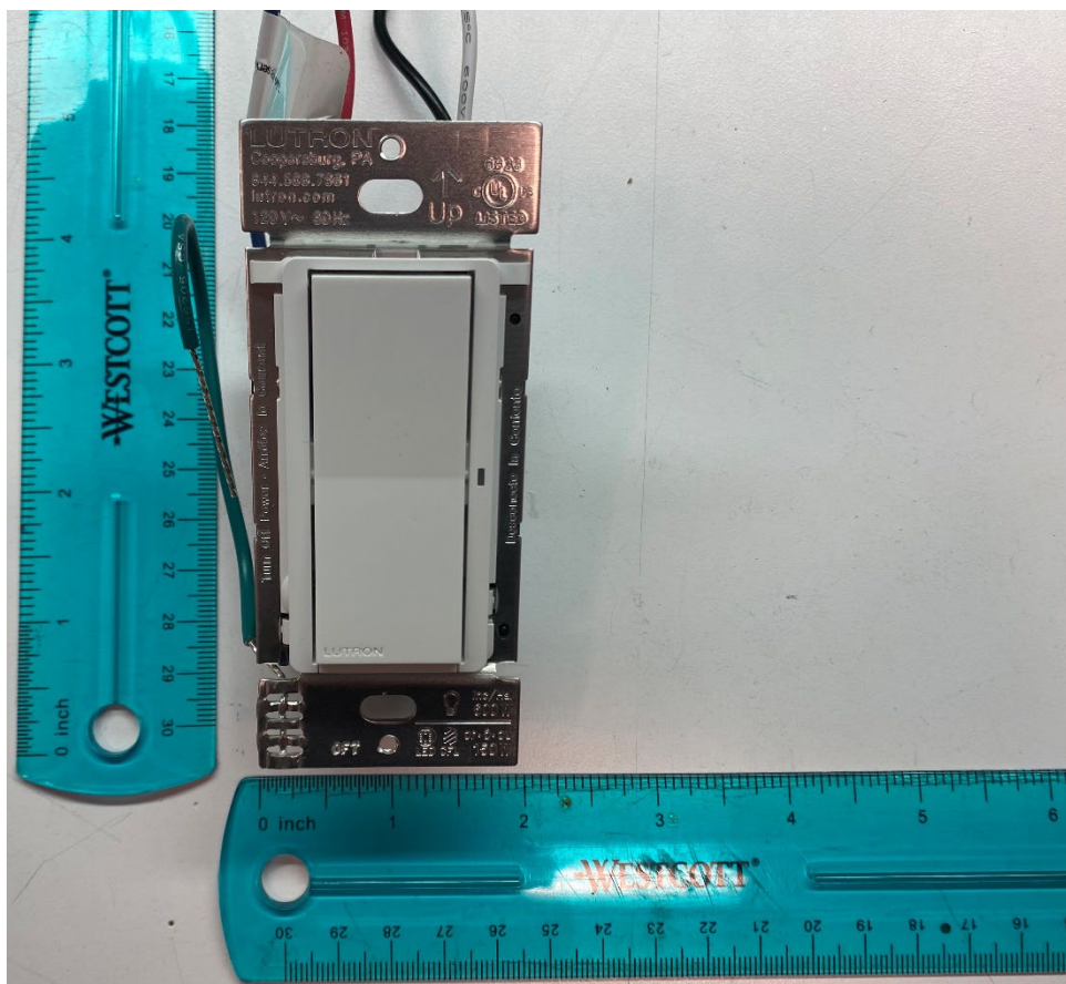
Front View
