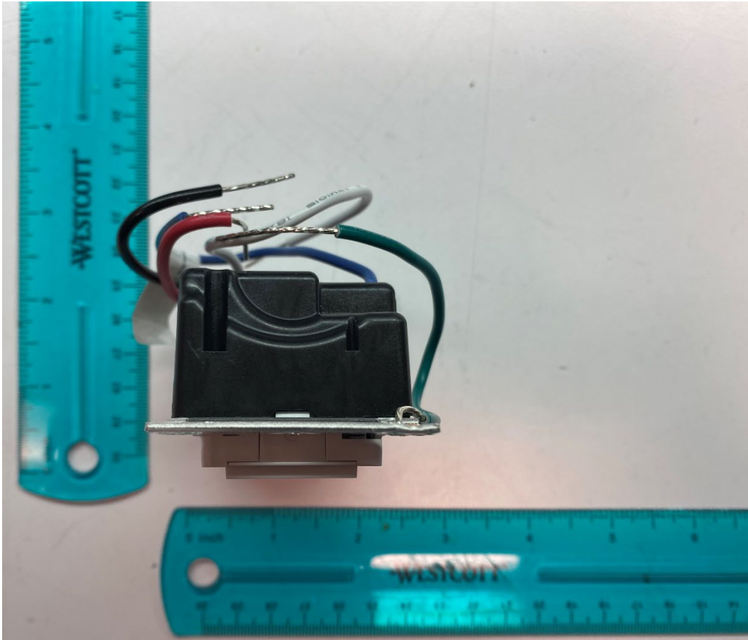
Bottom View
