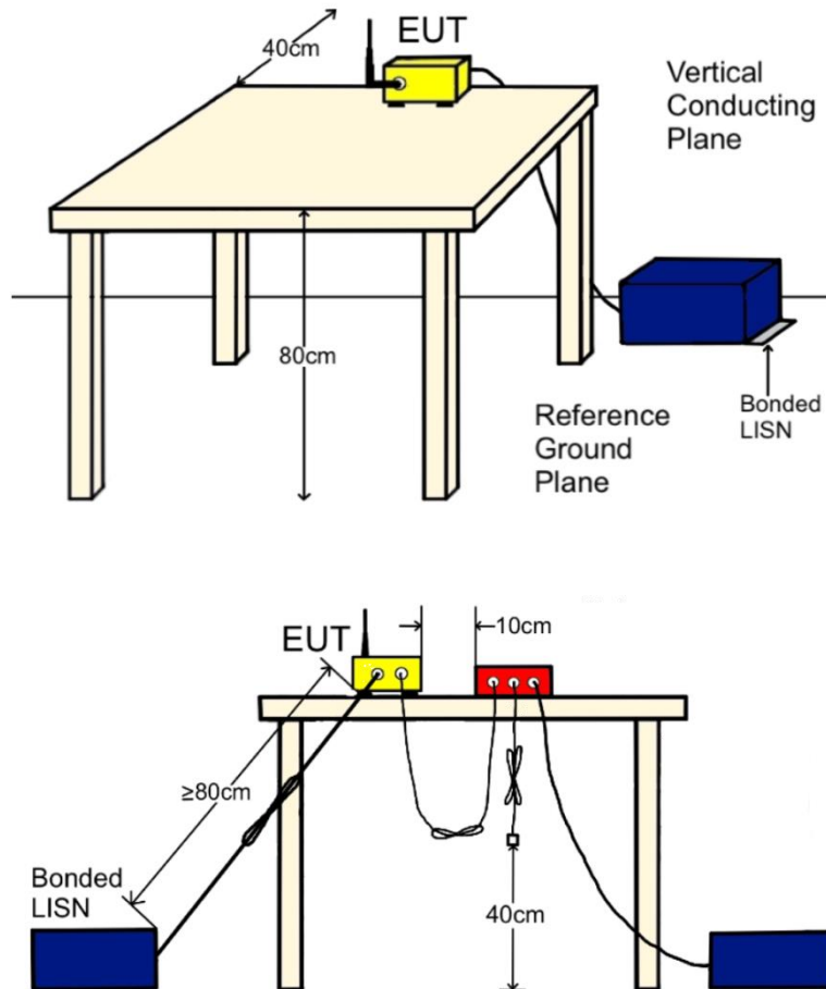
Figure 9: Conducted Emissions Test Setup
