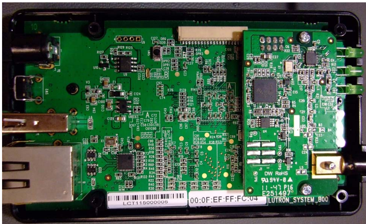
Figure 1: Internal with RF Board in place
