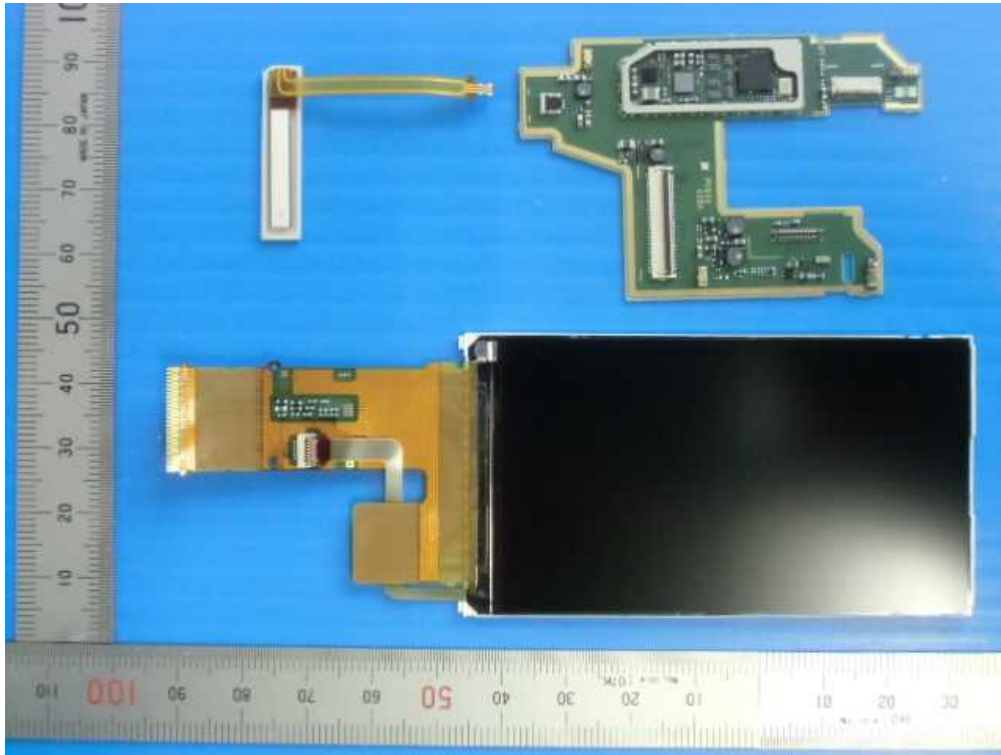
LCD PCB
