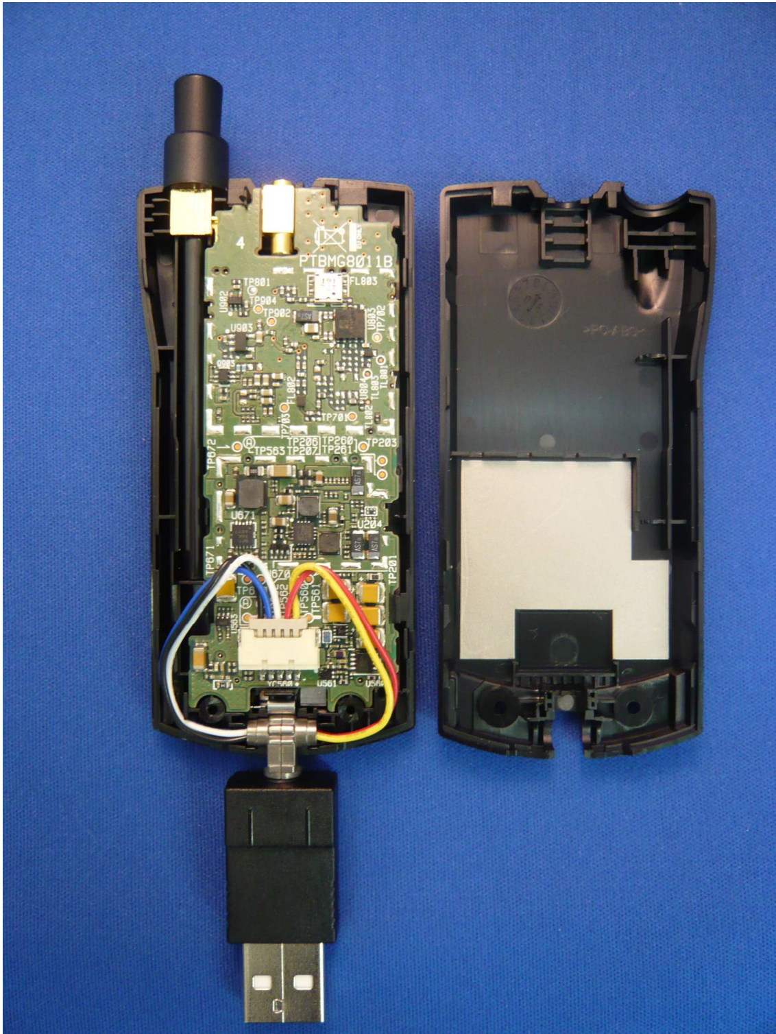
Main Board with Case
