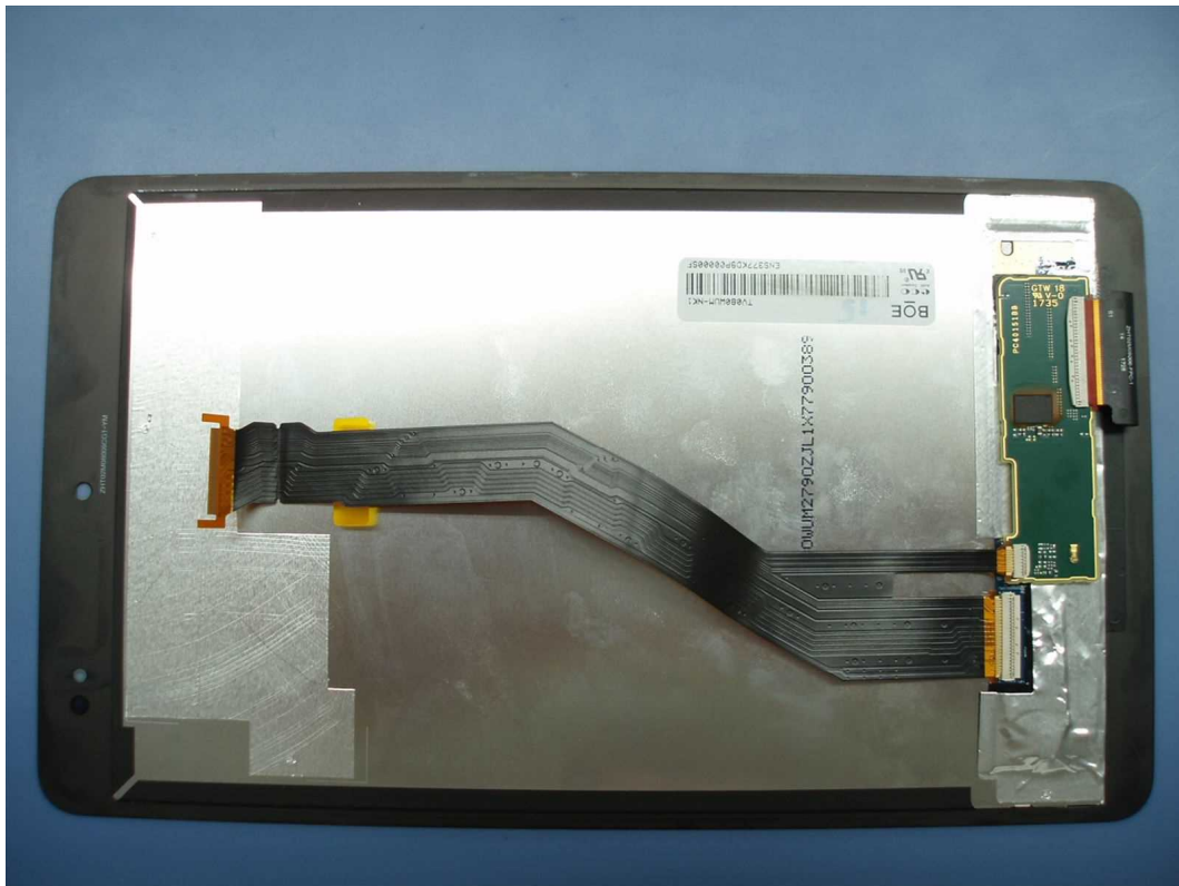
LCD rear
