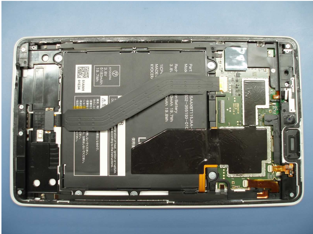
Main PCB
