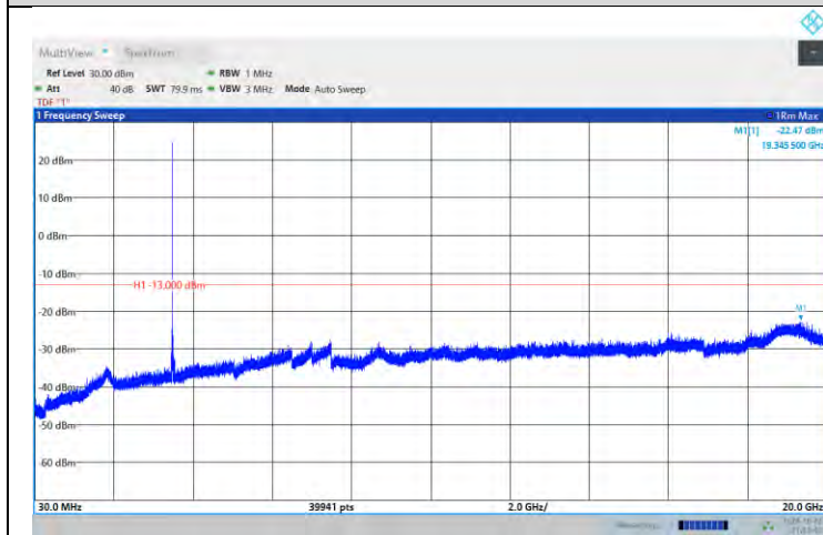
Band42-15MHz-64QAM-43015-1RB#0-Range:30~20000MHz
