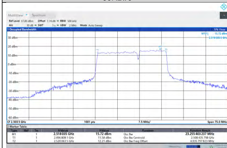
41-41-15MHz-10MHz-QPSK-QPSK-41417-41537-75RB#0-50RB#0
