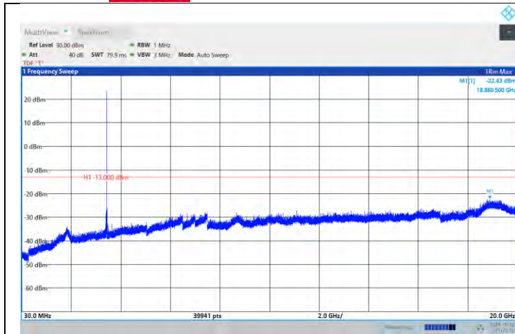
Band42-15MHz-64QAM-42590-1RB#0-Range:30~20000MHz
