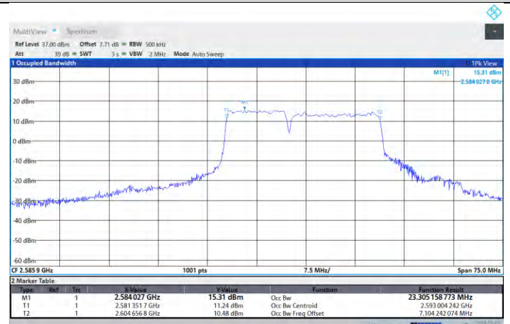
41-41-10MHz-15MHz-16QAM-16QAM-39703-39823-50RB#0-75RB#0
