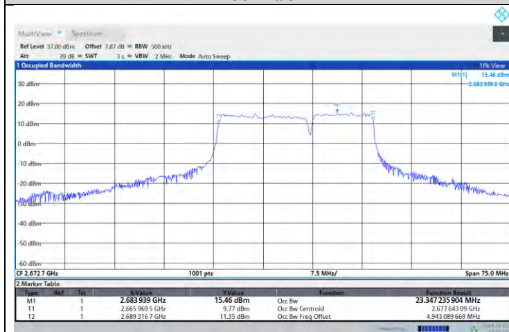
41-41-15MHz-10MHz-16QAM-16QAM-40571-40691-75RB#0-50RB#0
