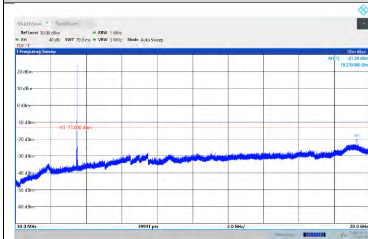
Band42-20MHz-64QAM-42990-1RB#0-Range:30~20000MHz
