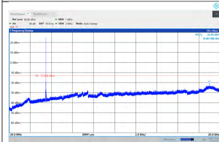
Band42-15MHz-16QAM-43015-1RB#0-Range:30~20000MHz
