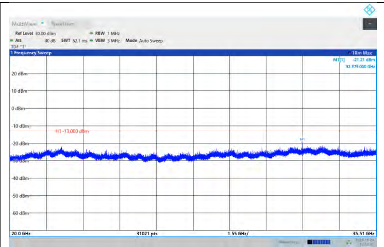
Band42-10MHz-QPSK-42590-1RB#0- Range:20000MHz~35510MHz
