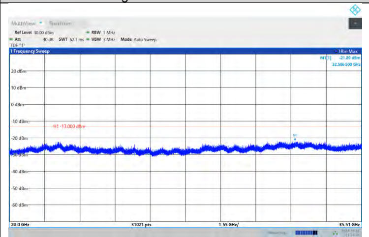
Band42-10MHz-QPSK-43040-1RB#0- Range:20000MHz~35510MHz
