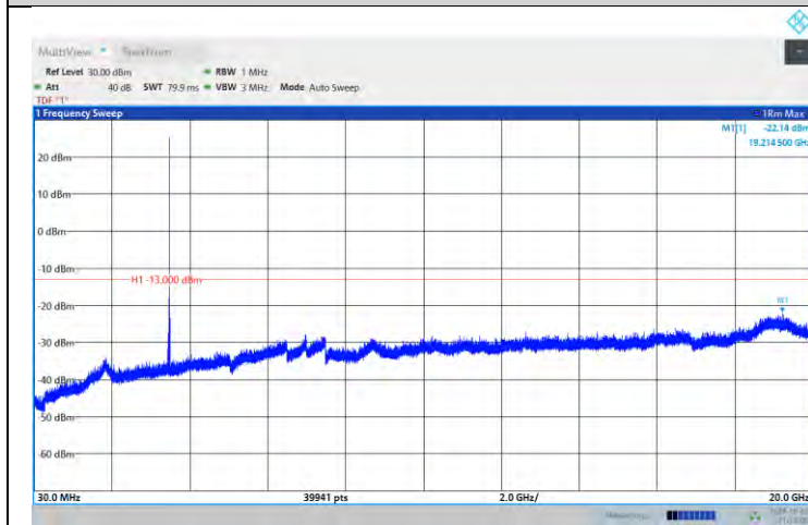
Band42-10MHz-QPSK-43040-1RB#0-Range:30~20000MHz
