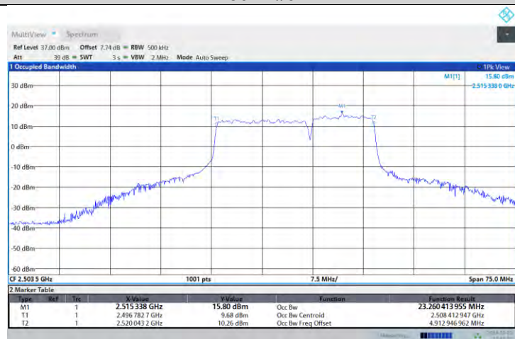
41-41-15MHz-10MHz-16QAM-16QAM-41417-41537-75RB#0-50RB#0
