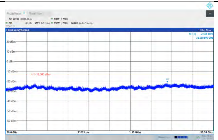
Band42-15MHz-64QAM-42590-1RB#0- Range:20000MHz~35510MHz
