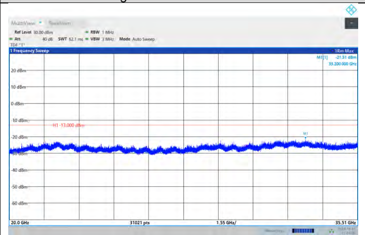
Band42-15MHz-64QAM-43015-1RB#0- Range:20000MHz~35510MHz
