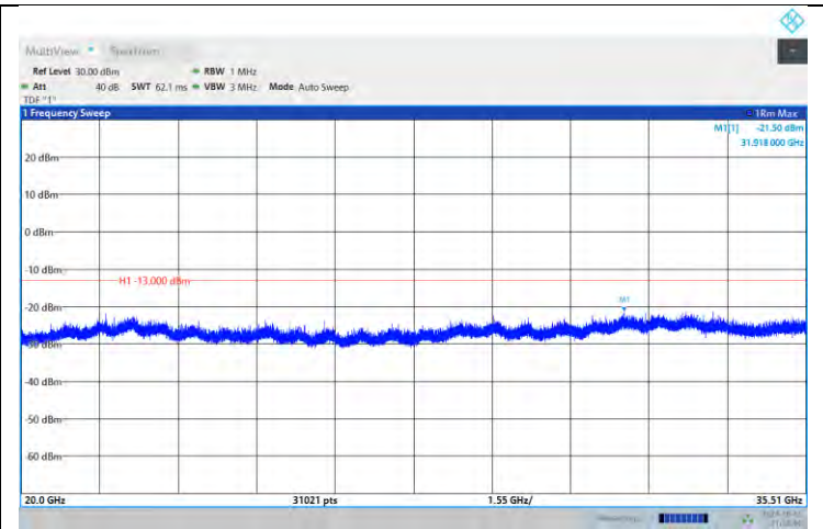
Band42-15MHz-16QAM-42590-1RB#0- Range:20000MHz~35510MHz
