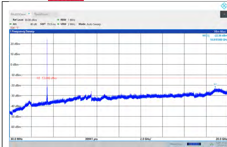
Band42-15MHz-16QAM-42590-1RB#0-Range:30~20000MHz
