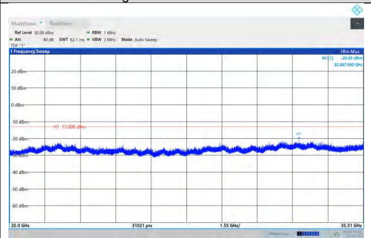
Band42-15MHz-16QAM-43015-1RB#0- Range:20000MHz~35510MHz
