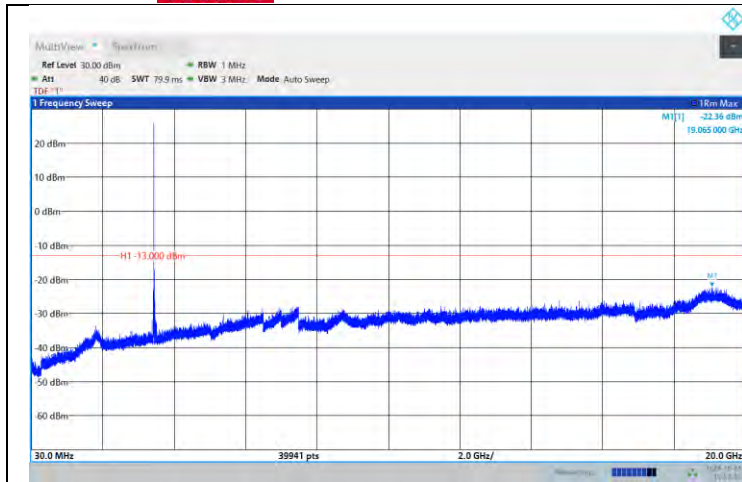
Band42-10MHz-QPSK-42590-1RB#0-Range:30~20000MHz
