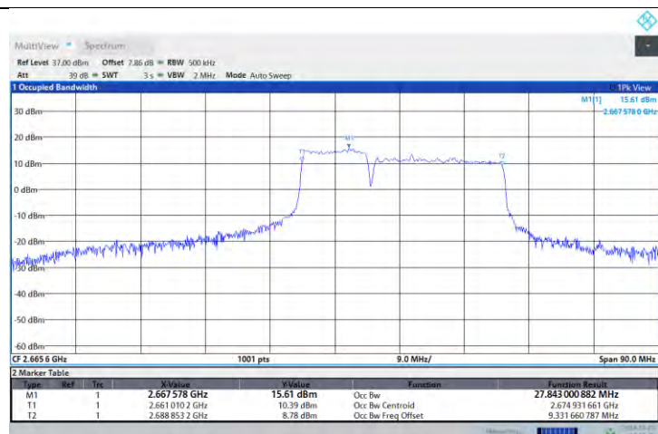
41-41-15MHz-10MHz-QPSK-QPSK-40571-40691-75RB#0-50RB#0
