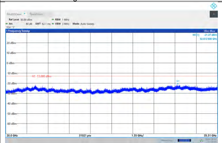
Band42-20MHz-64QAM-42990-1RB#0- Range:20000MHz~35510MHz
