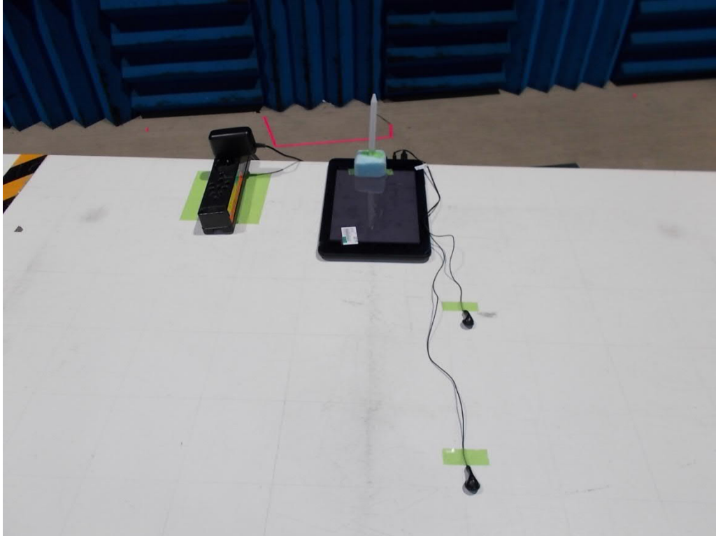
Pen setup
