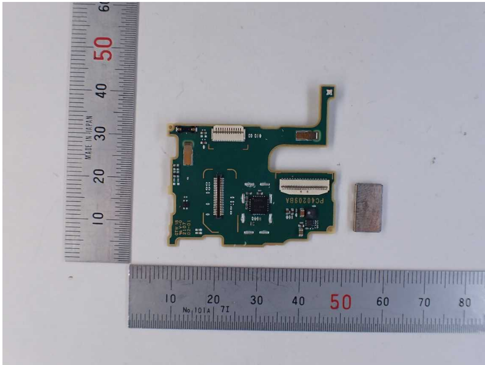
LCD PCB Front without shield
