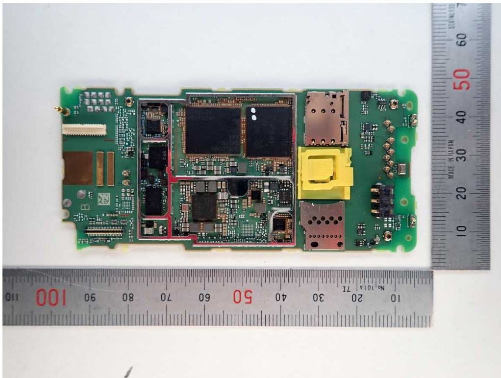
Main PCB Front without shield
