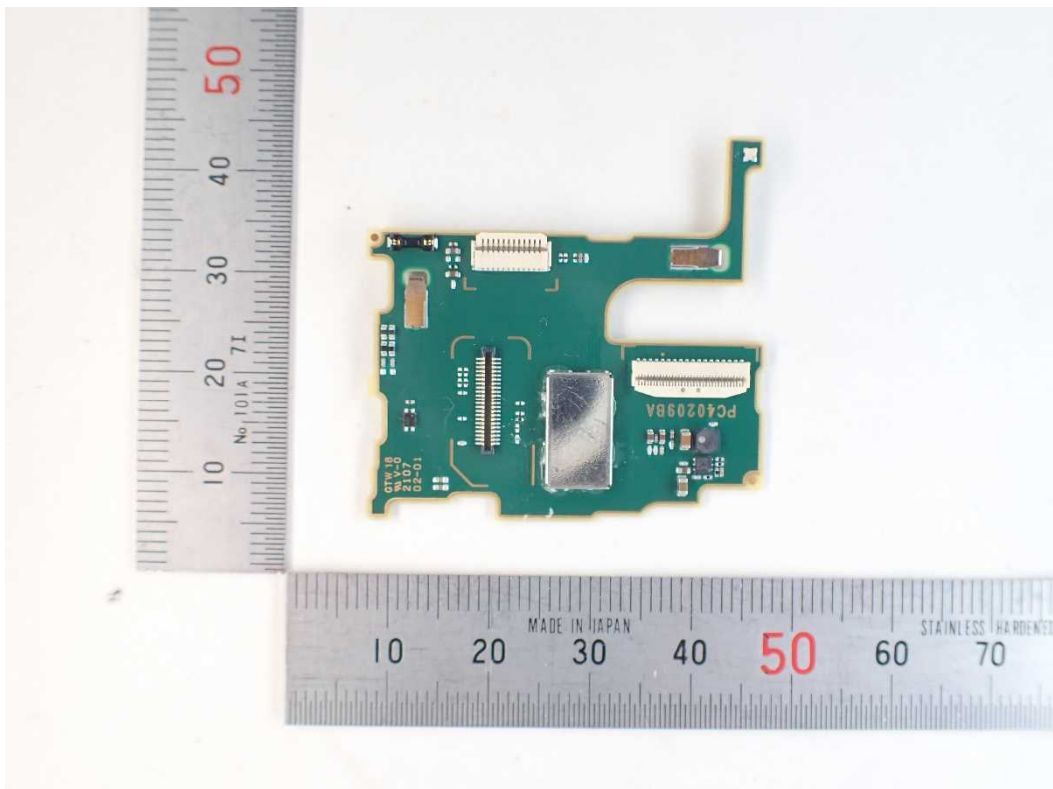
LCD PCB Front with shield
