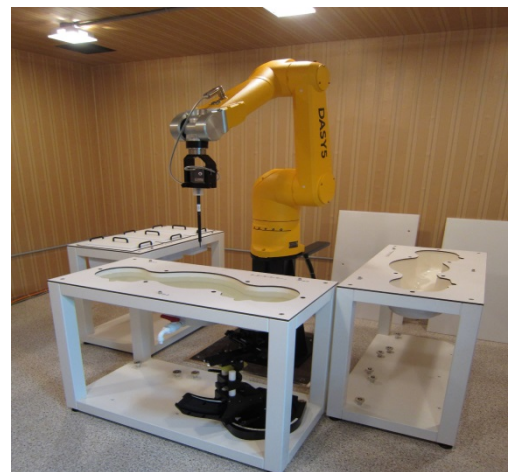
Figure 4.1 DASY5 Test System
