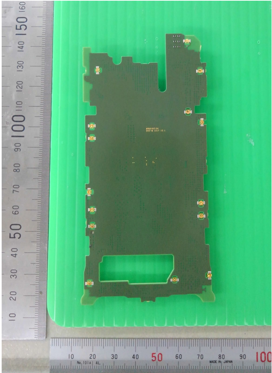
Main PCB back
