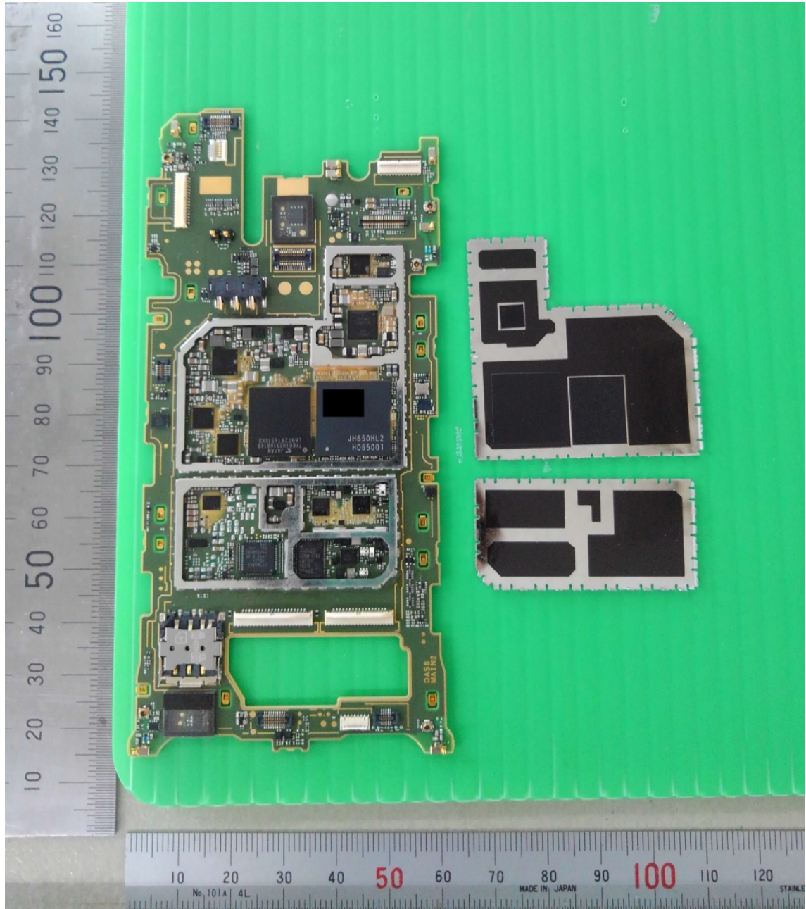
Main PCB front
