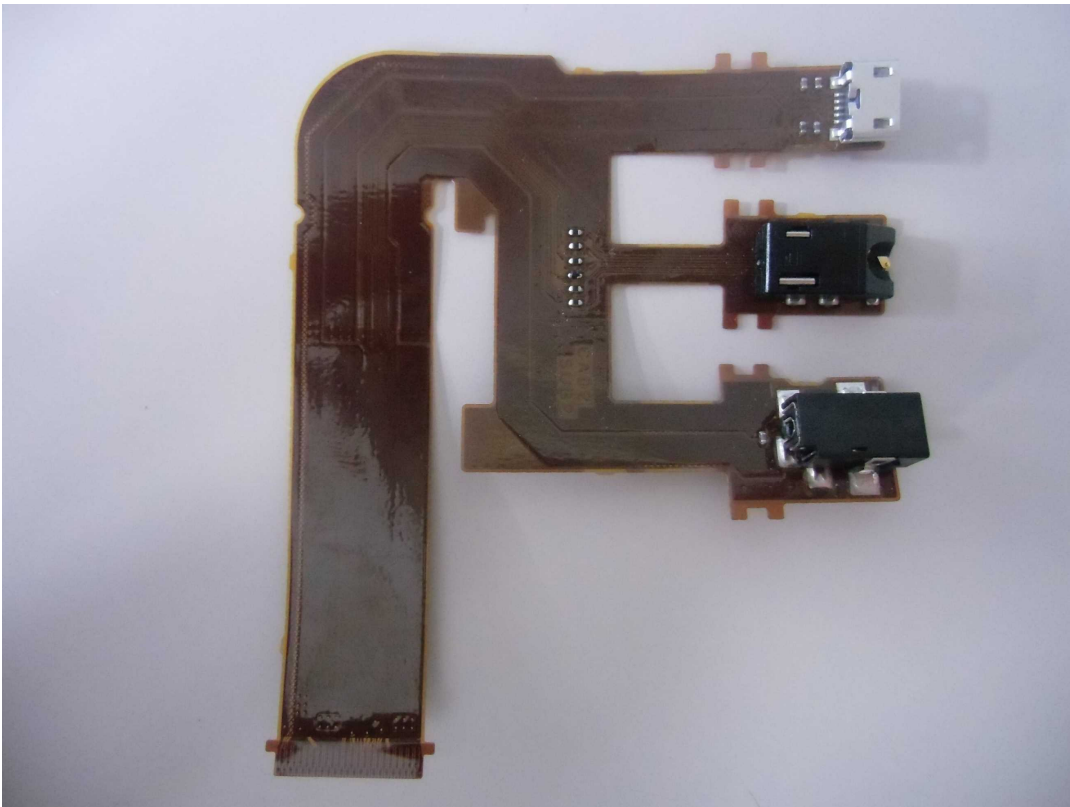
Sub FPC
