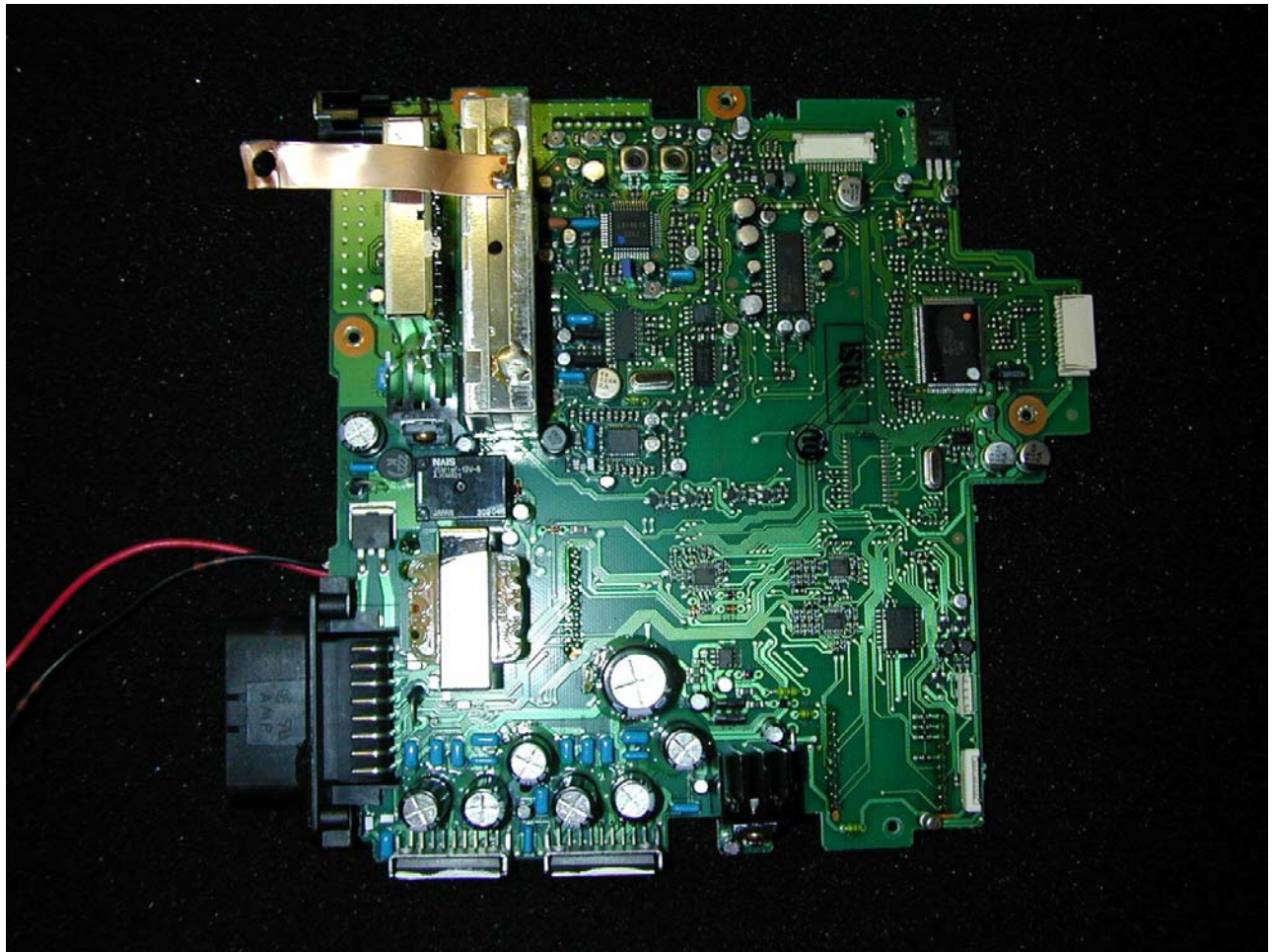
Figure 8 – Top PCB (Bottom)
