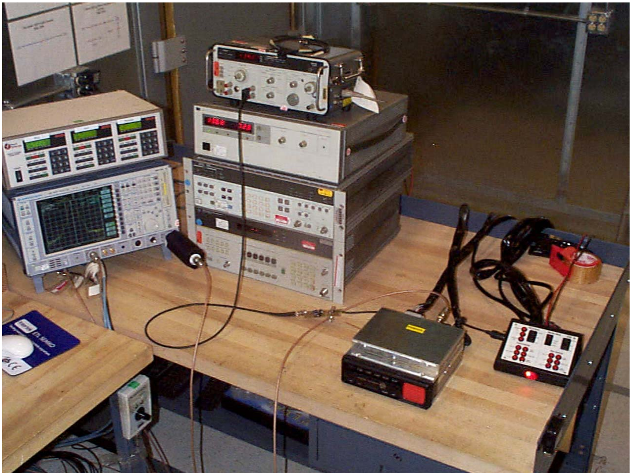
Figure 1 – Output Power, Occupied Bandwidth, and Conducted Spurious Emissions
