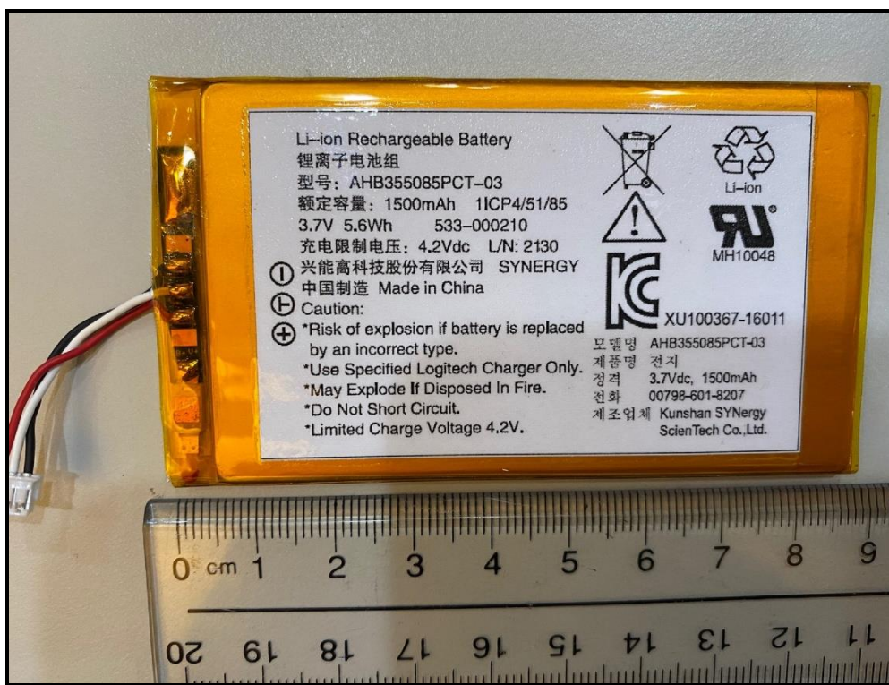
Battery 2 (Model: AHB355085PCT-03 or 533-000210)
