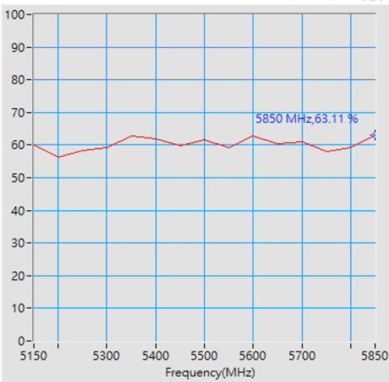
Maximum Efficiency at 5850 MHz : 63.11 %
