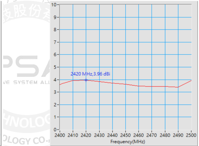
Maximum Peak Gain at 2420 MHz : 3.96 dBi
