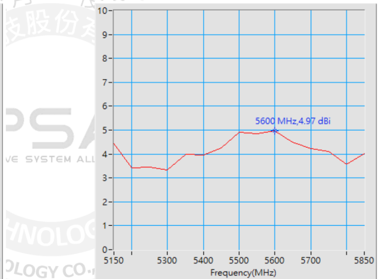
Maximum Peak Gain at 5600 MHz : 4.97 dBi
