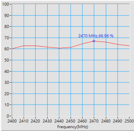
Maximum Efficiency at 2470 MHz : 66.96 %
