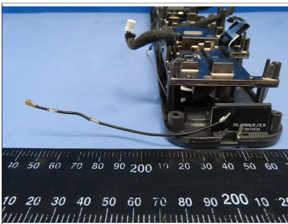
ANT_ Bluetooth
