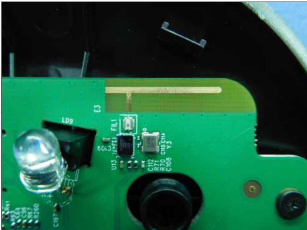
GFSK antenna
