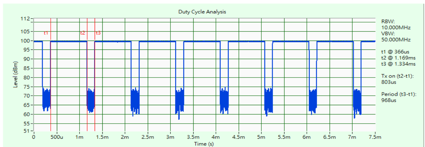
Time-domain plot for Bluetooth (SRD) transmission signal
