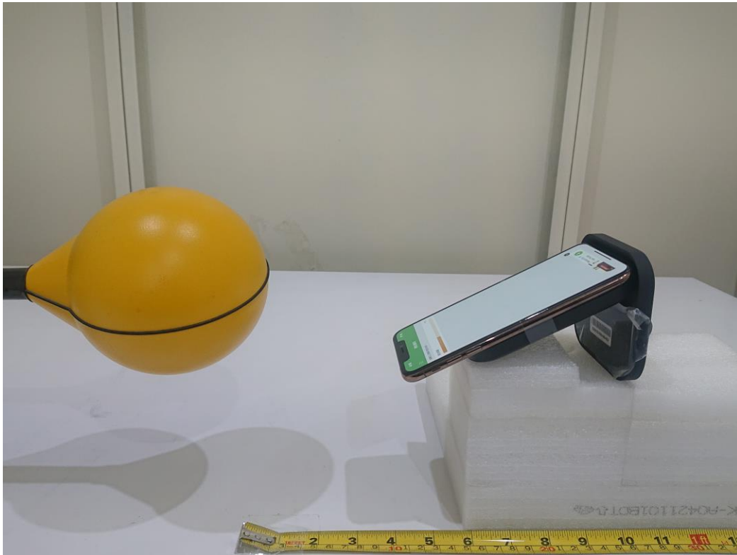
H-Field (Charging Mode – Z-axis)
