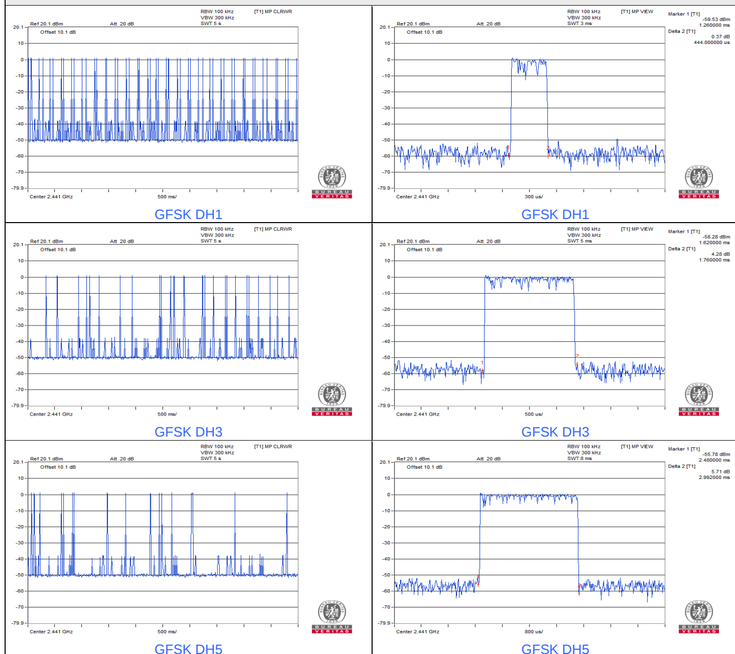
Spectrum plots of the transmitting time slot
