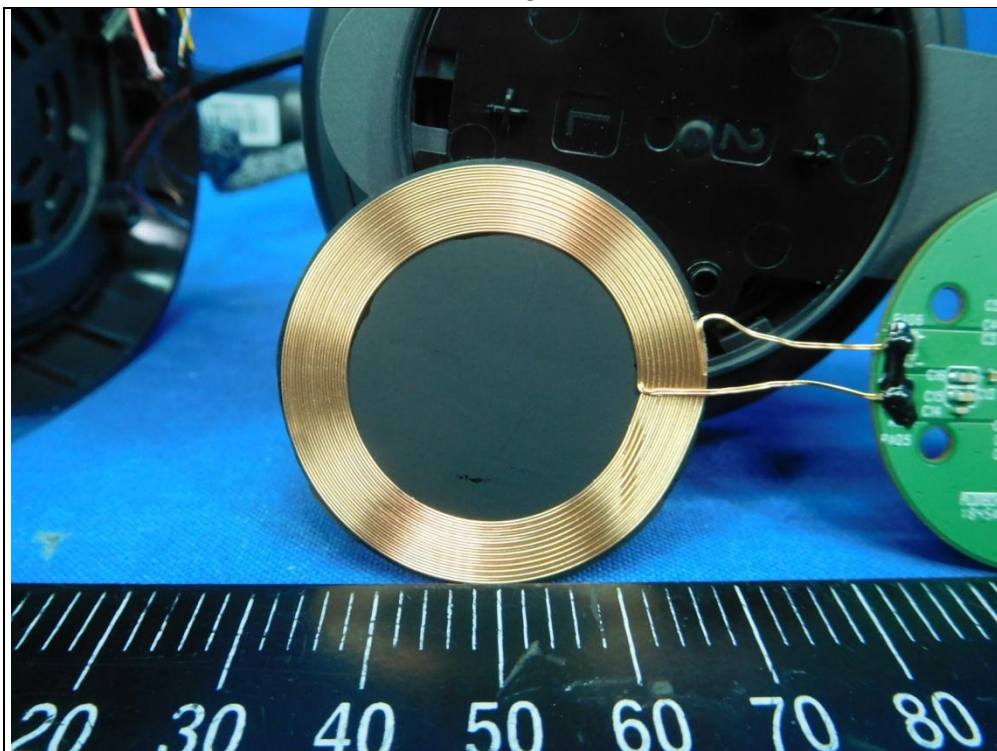
Wireless Charge Antenna
