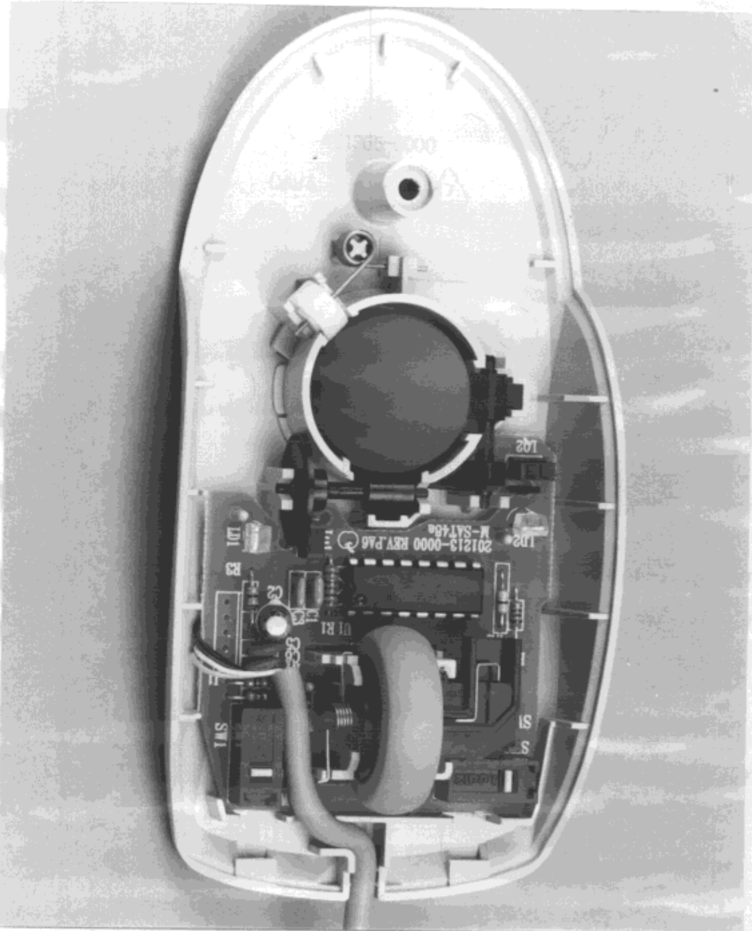
Photograph of EUT Construction (Model : M-SAT48A)
