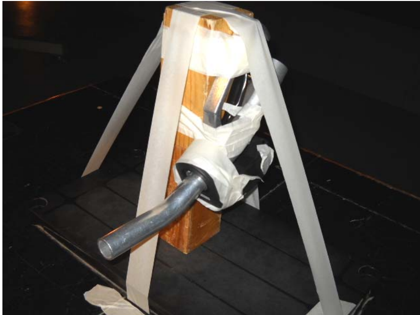
Photograph No.4 Radiated emissions measurement setup in the anechoic chamber close view
