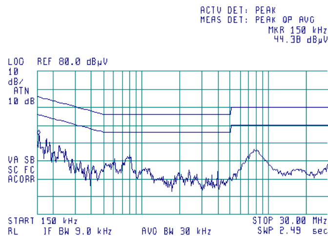
Plot 7.4.4 Conducted emission measurements with dummy load in lieu of the antenna
