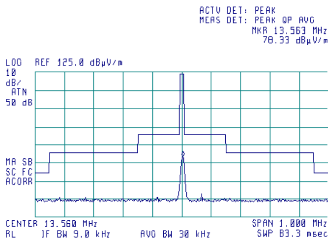
Plot 7.1.2 Fundamental emission test result at 115% U_{nom} input voltage
