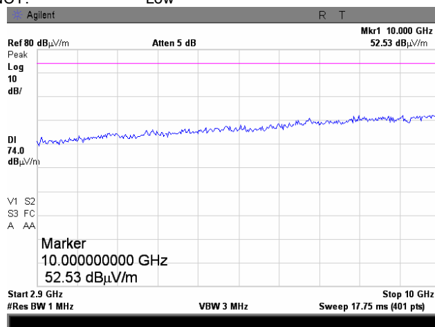
Plot 7.1.16 Radiated emission measurements from 2.9 to 10.0 GHz
