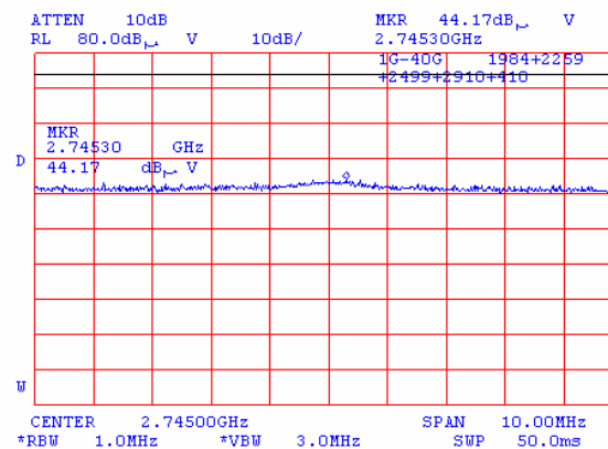
Plot 7.1.23 Radiated emission measurements at the third harmonic frequency
