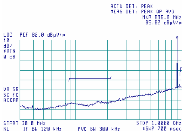
Plot 7.1.10 Radiated emission measurements from 30 to 1000 MHz
