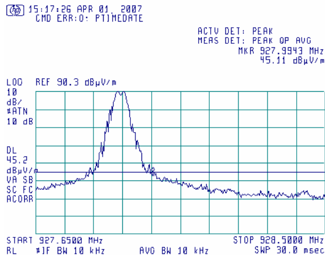
Plot 7.2.2 Hgh band edge emission test result
