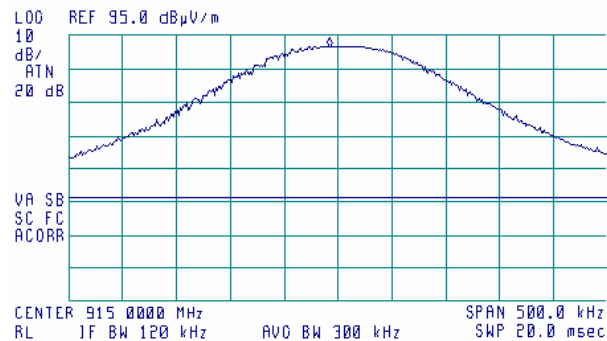
Plot 7.1.4 Radiated emission measurements at the fundamental frequency
