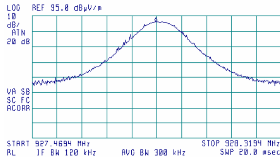
Plot 7.1.6 Radiated emission measurements at the fundamental frequency
