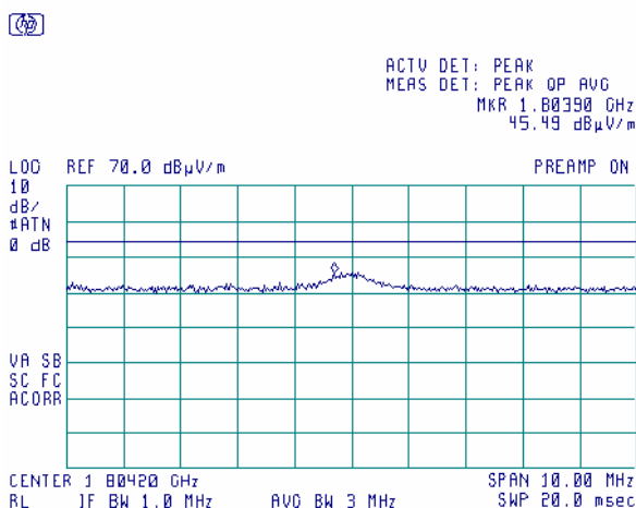
Plot 7.1.19 Radiated emission measurements at the second harmonic frequency
