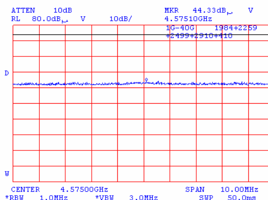
Plot 7.1.29 Radiated emission measurements at the fifth harmonic frequency
