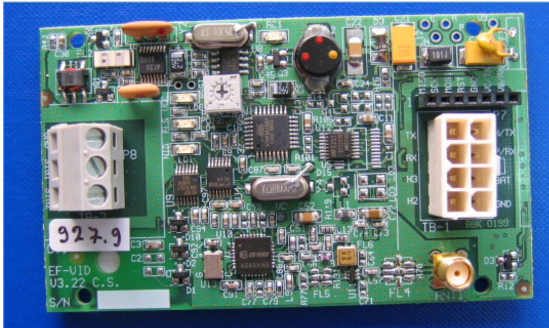
Photograph No.2 PCB front view
