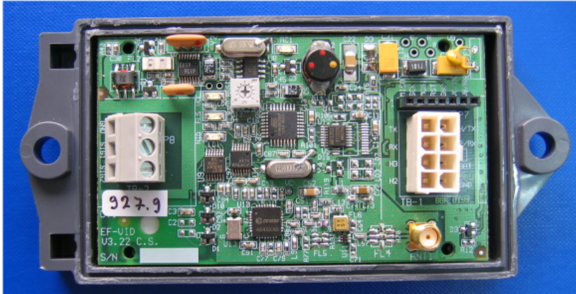
Photograph No.1 Vehicle identification unit internal view
