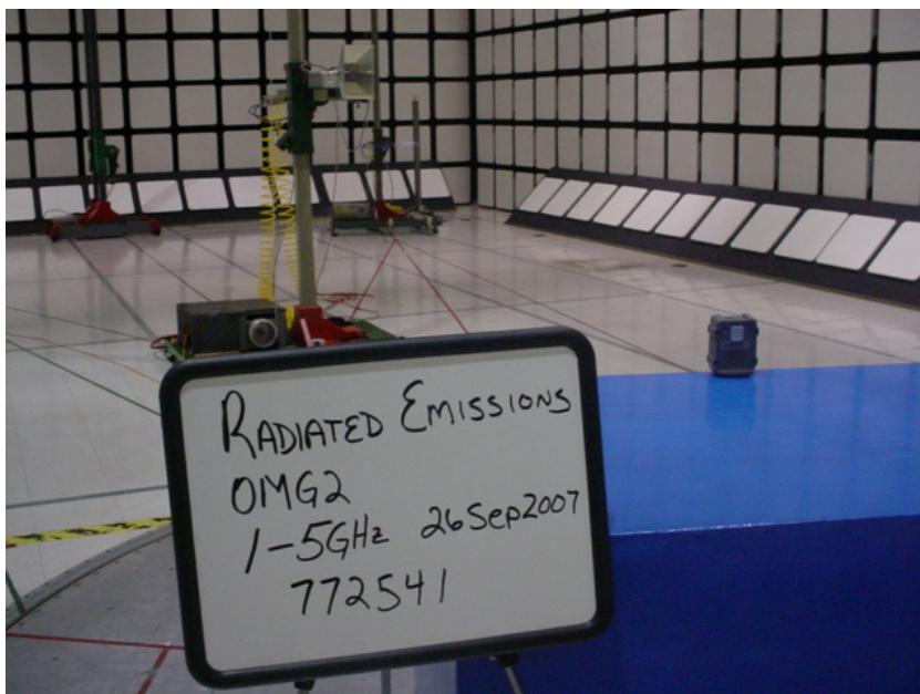
Figure 10 Test setup for Radiated Emissions (1-5GHz)
