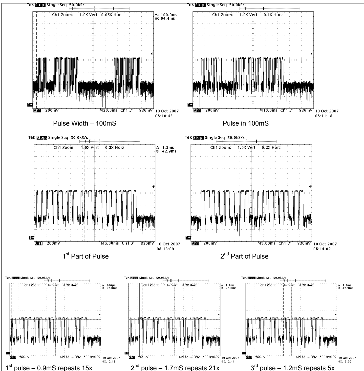
Figure 7 Pulse Train Graph
