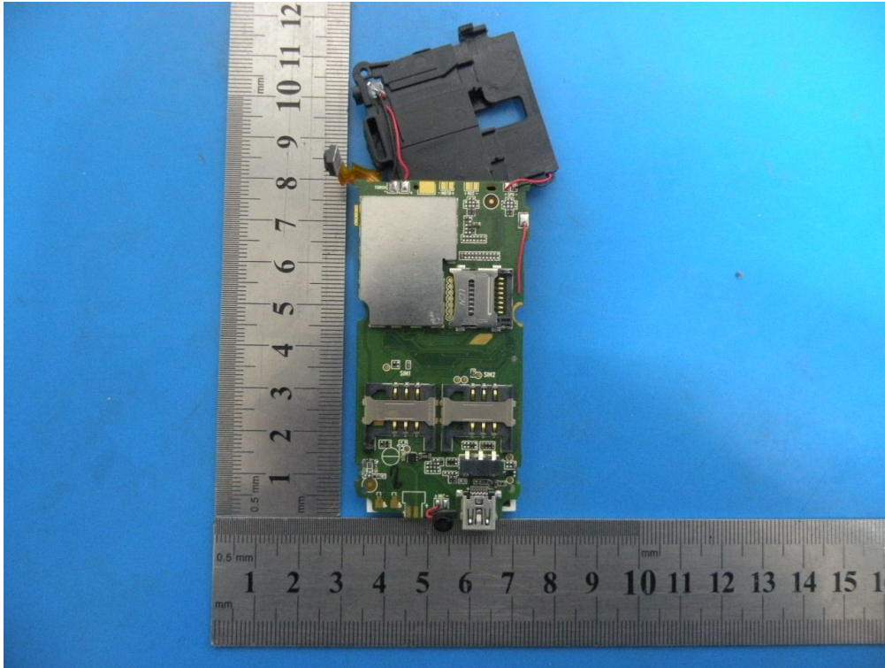
Bottom View
