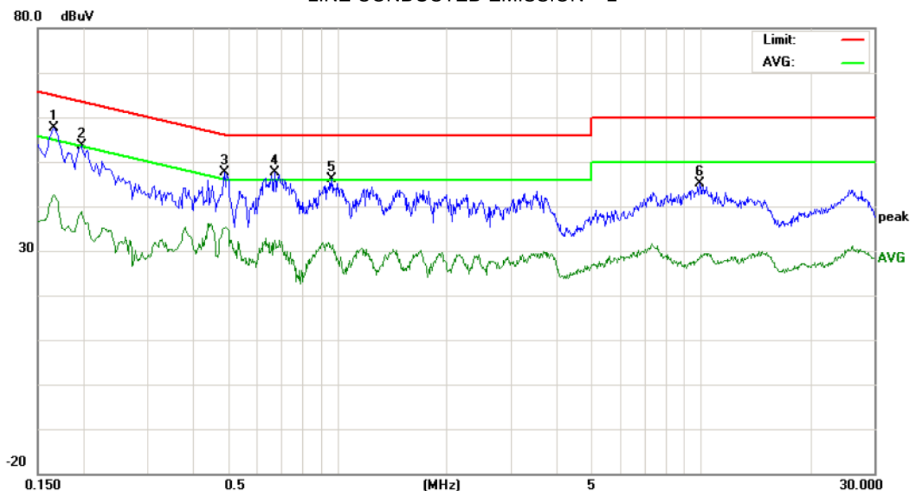
LINE CONDUCTED EMISSION – L
