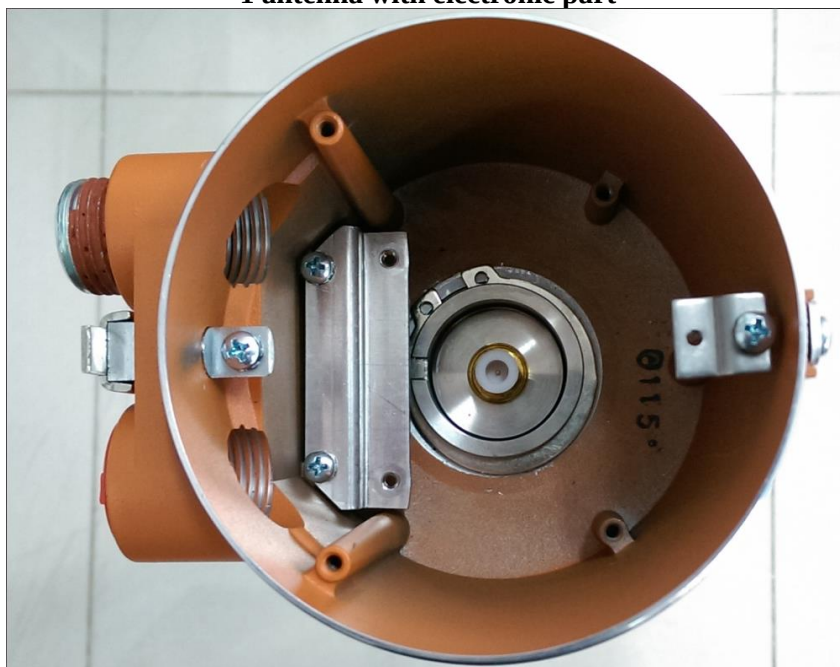
2 antenna with connector top view
