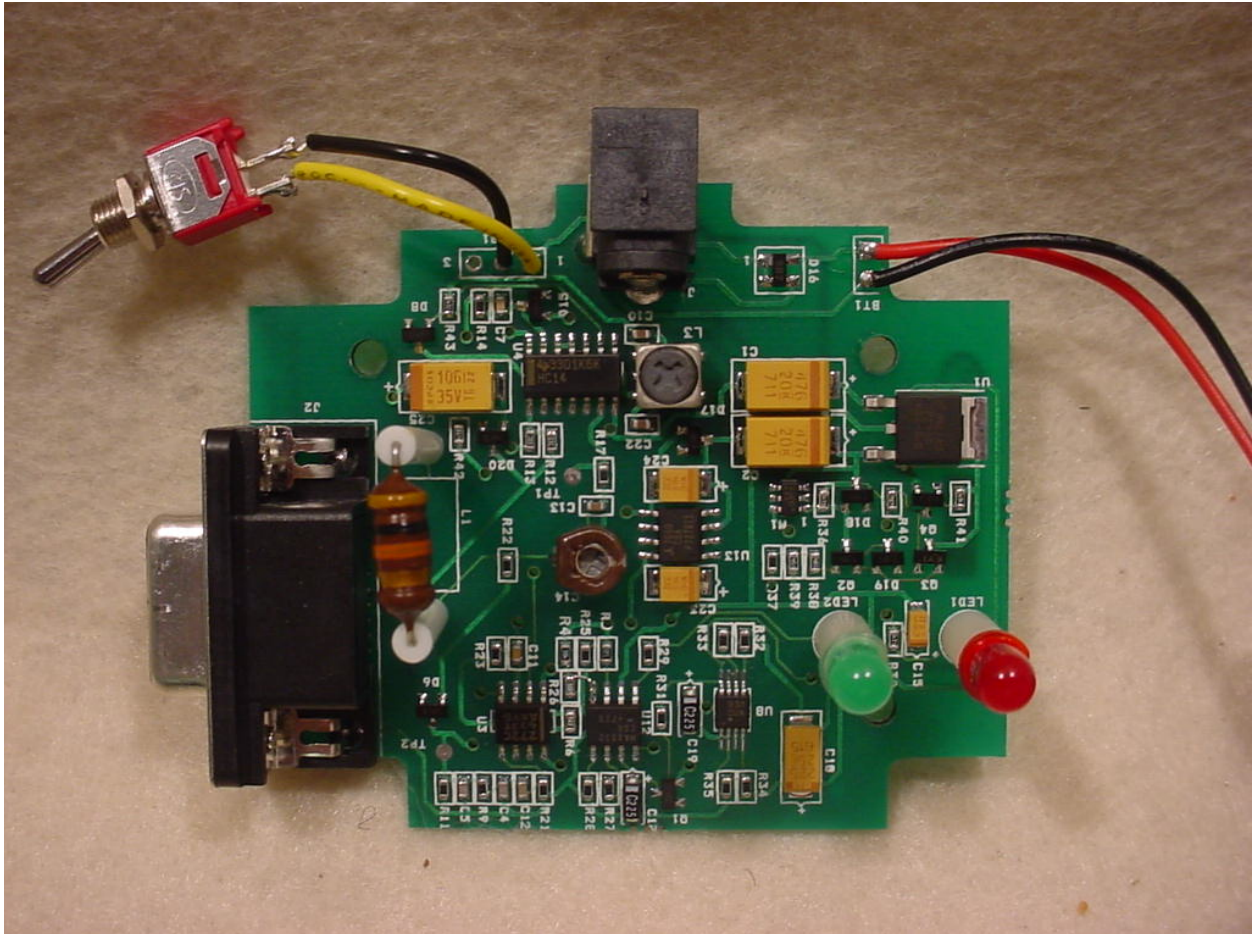
Figure 2: PCB Front
