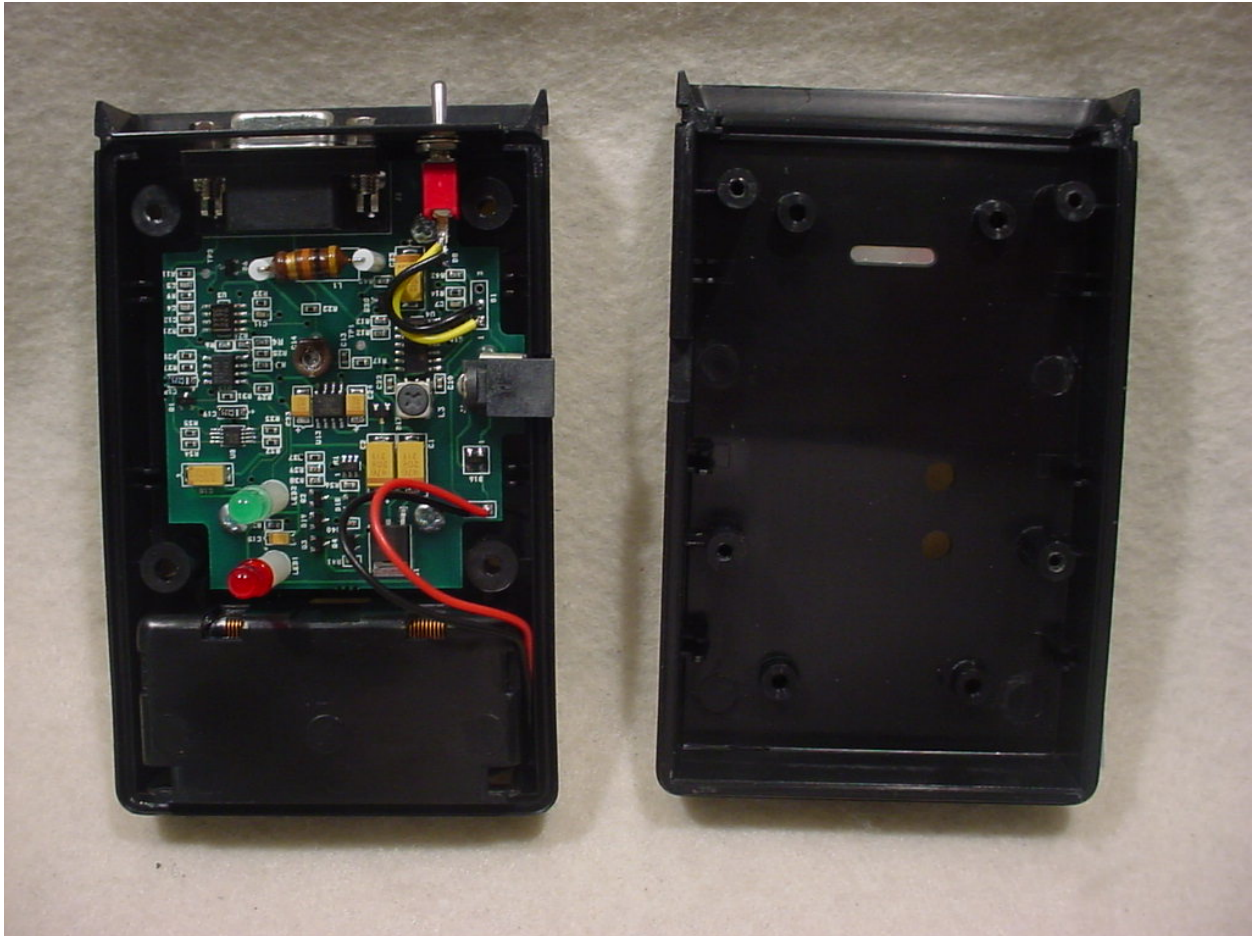
Figure 1: Assembled View
